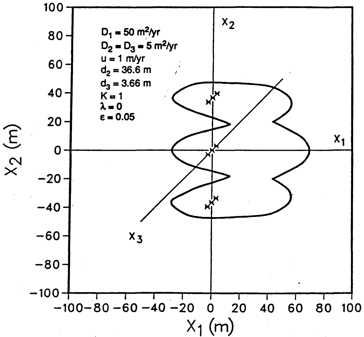
Figure 2 Isopleth of a contaminant at concentration 0.01 \text{ g}/\text{m}^3 for steady-state, anisotropic dispersion for the array of point sources in Figure 1
