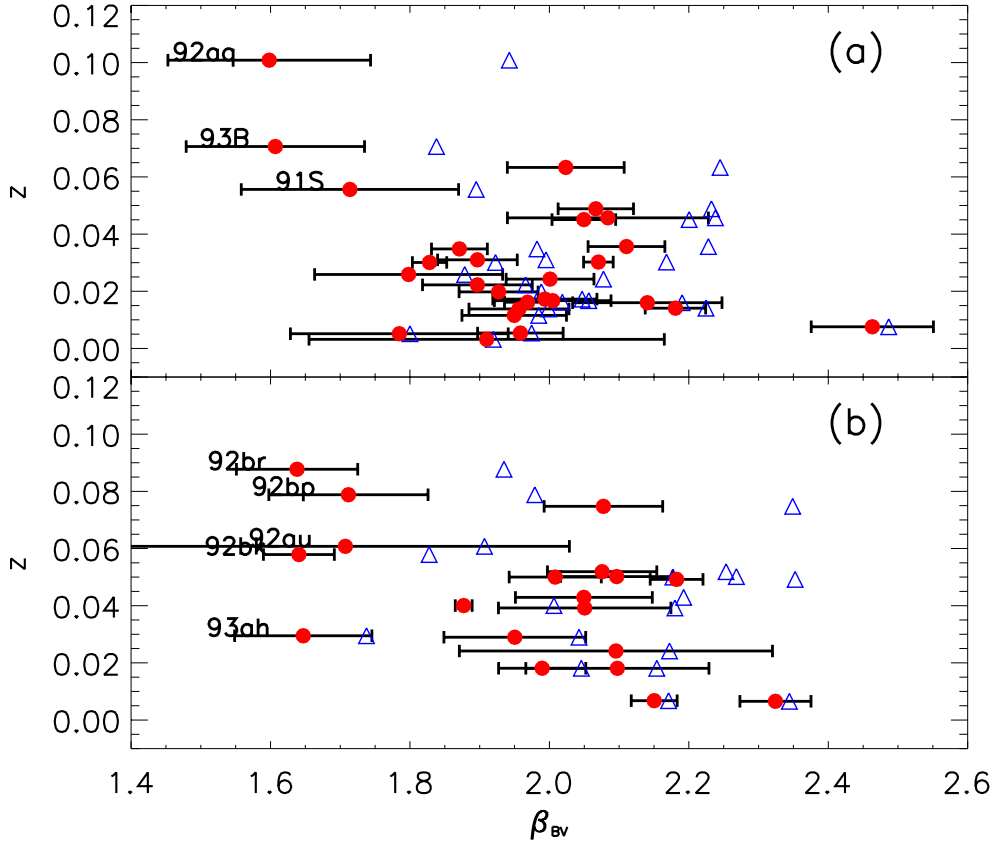
Fig. 9.— Redshift versus slopes with (filled red circles ) and without (blue triangles) K-corrections for supernovae from spiral (a) and E+S0 (b) galaxies. The secondary enhancement at \beta_{BV} = 1.65 shown in Figure 7(b) is also apparent in (b). The data are suggestive of different branches of supernovae with intrinsically different slopes, but more data are needed to test such differences.
