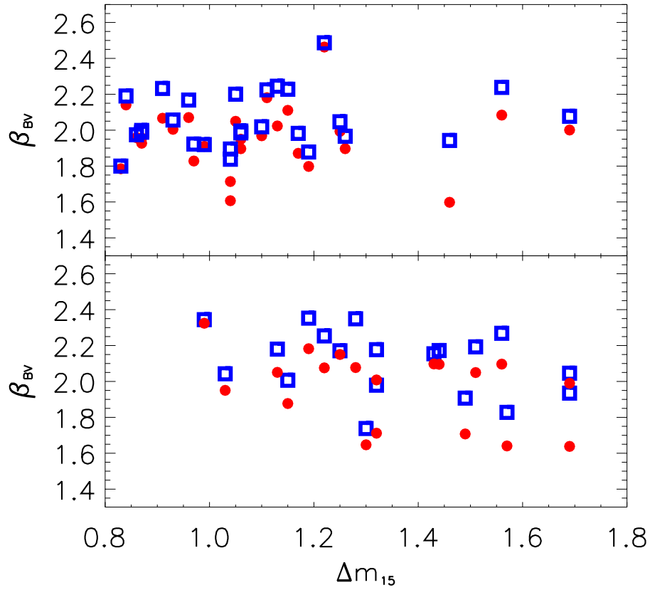
Fig. 8.— The slopes of the Color-Magnitude fits versus the light curve decline rate \Delta m_{15} for supernovae from spiral (upper panel) and E+S0 (lower panel) hosts. Red circles are for the slopes after K -corrections, and blue squares are the data without K -corrections. No correlation is seen between the slopes and \Delta m_{15} , as is expected from the definitions in equation 2.
