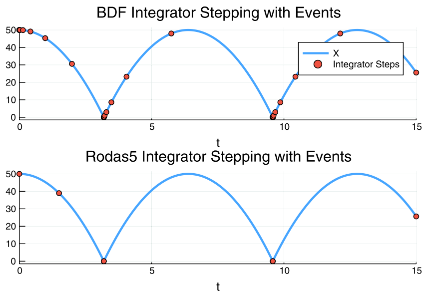
Fig. 2. BDF integrator time stepping with events. Shown is the solution of the bouncing ball hybrid ODE system v' = -g , x' = v where g is the gravitational constant 9.8 and the sign of v flips whenever x = 0 . In the case of the BDF integrator (SUNDIALS 3.1), events cause a reset of the order of the integrator to 1, causing 39 time steps to be taken (shown in orange). Meanwhile, the Rodas5 integrator (OrdinaryDiffEq.jl) solves the equation in 5 time steps, jumping from event to event and utilizing an interpolation to fill in the intermediate region.
