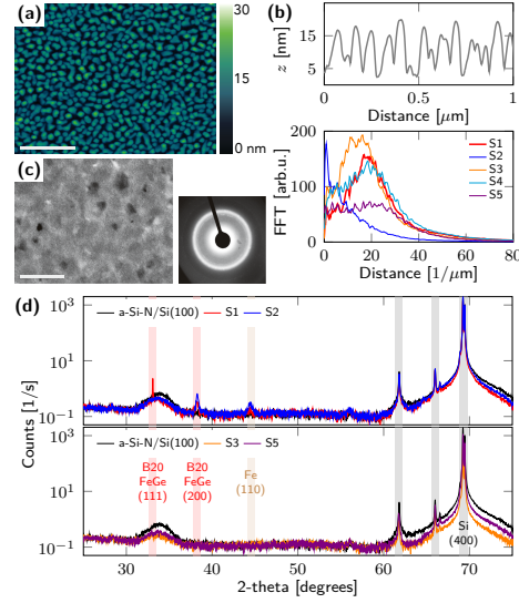
Figure 1. Structural properties of nanogranular iron germanium films on silicon nitride substrates and membranes characterized using (a,b) atomic force microscopy, (c) transmission electron microscopy, and (d) x-ray diffraction. Scale bar is (a) 500 nm and (c) 100 nm. (b) Line profile and angle-averaged Fourier transform to determine the grain size. (c) Selected-area electron diffraction using a 10- \mu\text{m} pinhole revealing an isotropic distribution of nanocrystalline grains. Microscopy data are shown for S1. (d) Two-theta x-ray diffraction scans confirming growth of (top) B20 FeGe nanocrystals within an amorphous structure and (bottom) pure amorphous structure.
