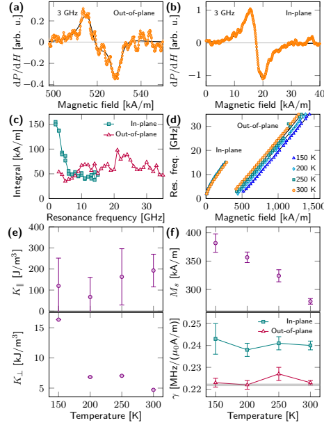
Figure 3. Ferromagnetic resonances in S1 films on silicon nitride substrates. (a) Out-of-plane and (b) in-plane ferromagnetic resonance spectra taken at 150 K consisting of multiple nearby resonances. The in-plane and out-of-plane resonance is fitted using one and two derivatives of the sum of symmetric and asymmetric Lorentzians, respectively. (c) Integrated power absorption derivative. (d) Dependence of the ferromagnetic resonance on magnetic bias field. (e) In-plane and out-of-plane magnetic anisotropy corroborating lateral isotropic strain and a preferential in-plane easy-plane spin orientation. (f) Saturation magnetization substantially larger than the magnetometry value and temperature-independent anisotropic gyromagnetic ratio \gamma . Horizontal line indicates free-electron value ( m_o = 0 ).
