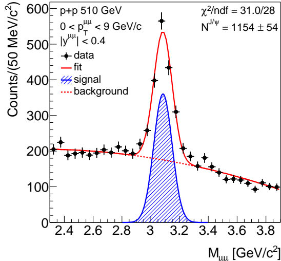
FIG. 1. The \mu^+\mu^- invariant mass spectrum in proton+proton collisions at \sqrt{s} = 510 GeV. The red solid line depicts a fit using a Gaussian function (blue line) for J/\psi signal and a second-order polynomial function (red dashed line) for background.
