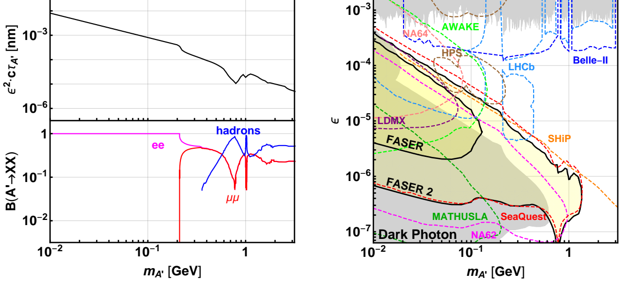
FIG. 6. Benchmark Model V1. The dark photon decay length (top left panel), its branching fractions into hadronic and leptonic final states (bottom left panel) and FASTER’s reach (right panel). In the right panel, the gray-shaded regions are excluded by current bounds, and the projected future sensitivities of other experiments are shown as colored contours. See the text for details.
