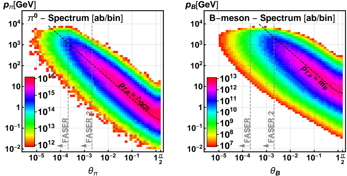
FIG. 5. Differential meson production rate in each hemisphere in the (\theta, p) plane, where \theta and p are the meson’s angle with respect to the beam axis and momentum, respectively. The bin thickness is 1/10 of a decade along each axis. We show the \pi^0 spectrum (left), obtained via EPOS-LHC [42], and the B meson spectrum (right), obtained using FONLL with CTEQ6.6 [44]. The diagonal black dashed lines highlight the characteristic transverse momentum scale p_T \sim \Lambda_{\text{QCD}} \sim 250 MeV for pions and p_T \sim m_B for B mesons. The angular acceptances for FASER and FASER 2 are indicated by the vertical gray dashed lines.
