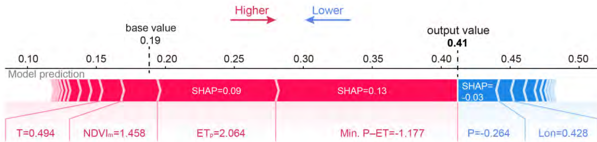
Figure S13. Explanation of an individual ET prediction at a 30-m pixel using SHAP. Red features (with positive SHAP values) push the ET output higher than the base value (i.e. toward the right), and blue features (with negative SHAP values) push the output lower. Base value represents the predicted ET without any feature knowledge, i.e. mean value obtained over 20,000 data points during the 2012-2015 drought. Input feature values are scaled and shown by z-score. In this case, historical-minimum P-ET is the primary driver of ET prediction.
