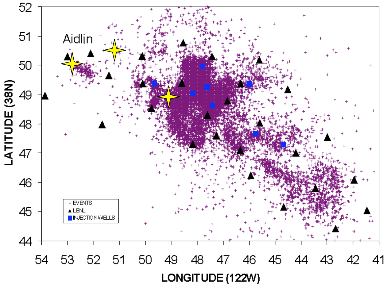
Figure 12. Locations of all events from October 2005 through August 2006, Geysers wide, note the increased clustering of events in the Aidlin area after injection has occurred. The blue boxes are the injection wells for the Santa Rosa water injection. The stars are magnitude 4 plus events (May 2006).
