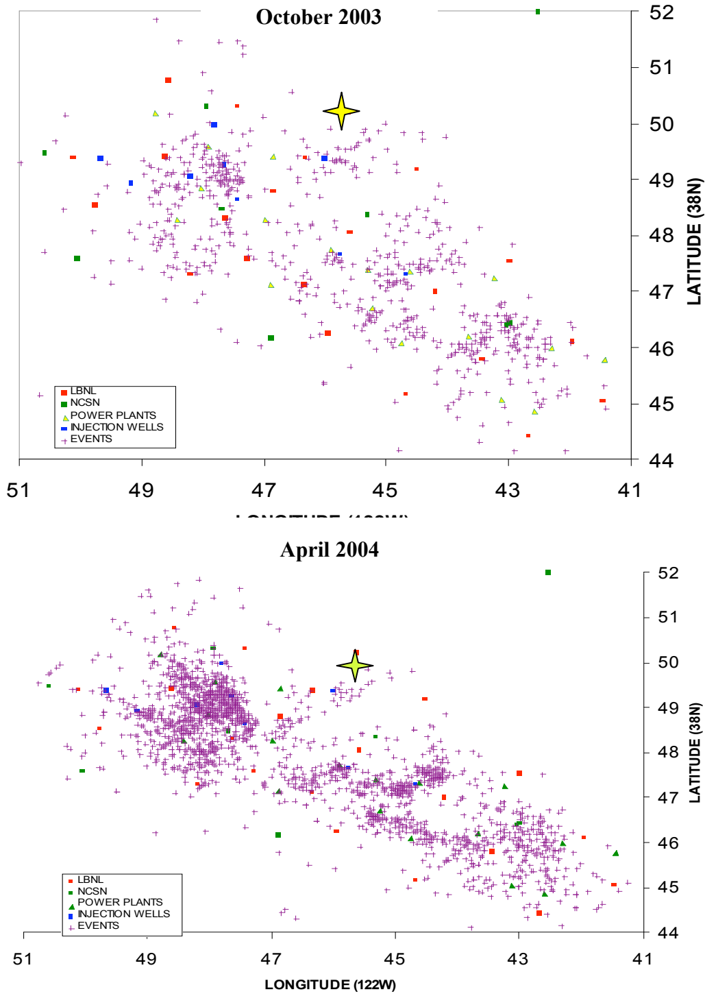
Figure 9. Top figure is one month of data recorded on the LBNL array before the Santa Rosa injection (October 2003) The bottom figure is one months of data (April 2004) after the Santa Rosa injection started. The star is the location of a February 2005 magnitude 4 event.
