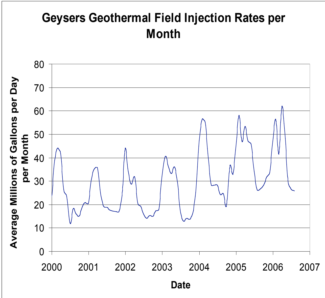
Figure 8. Total injections per day, averaged per month from 2000 through mid 2006 in millions of gallons for the entire Geysers field.
