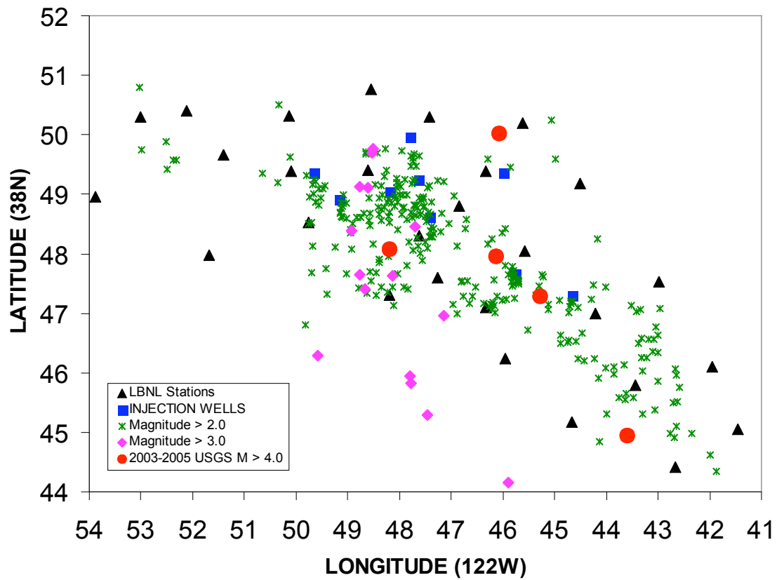
Figure 11. Location of magnitude 2, 3 and 4's from October 2003 through October 2005. The injection wells are only for the Santa Rosa water.
