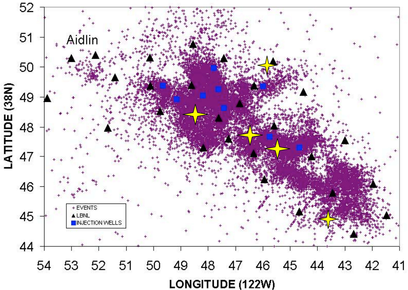
Figure 10. Locations of all events from October 2003 through October 2005, Geysers wide, note the relatively lack of events in the Aidlin area, this is prior to a large increase in injection in the Aidlin area, injection started in late 2005. The blue boxes are the injection wells for the Santa Rosa water injection. The large stars are magnitude 4 plus events (Feb. 2004, Dec. 2004, May 2005, Oct. 2005). The linear trends in the data are artifacts of the automatic location.
