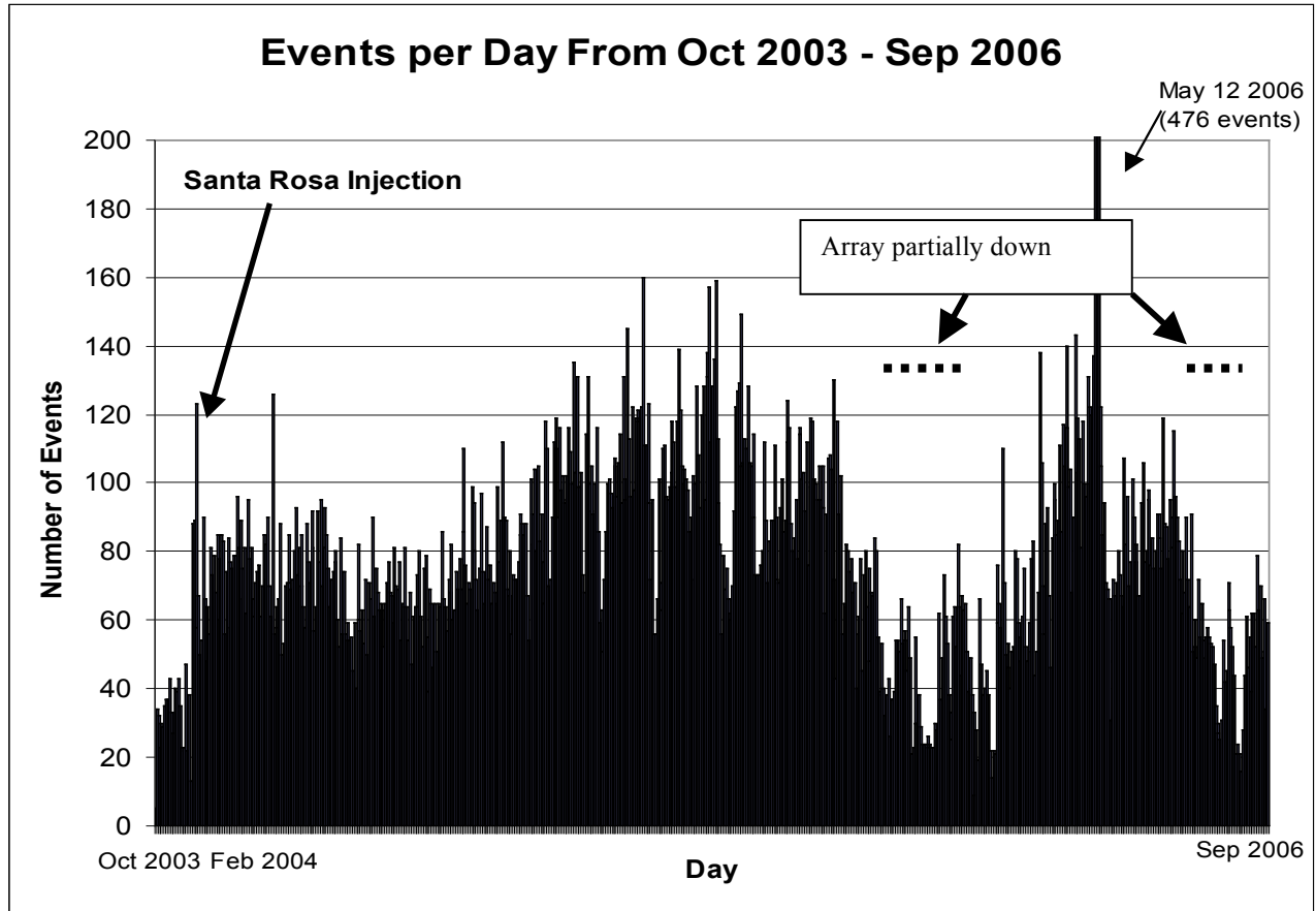
Figure 7. The rate of seismicity before and after the Santa Rosa injection as recorded by the LBNL array, the start of injection was December of 2003. The times marked with the array partially down was due to fires destroying parts of the array.
