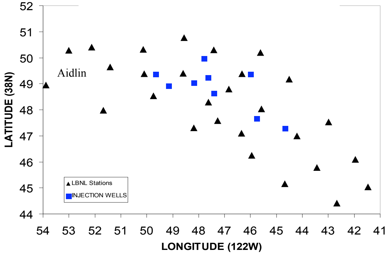
Figure 3. The entire current array including the Aidlin stations, the squares are the injection wells for the Santa Rosa water.
