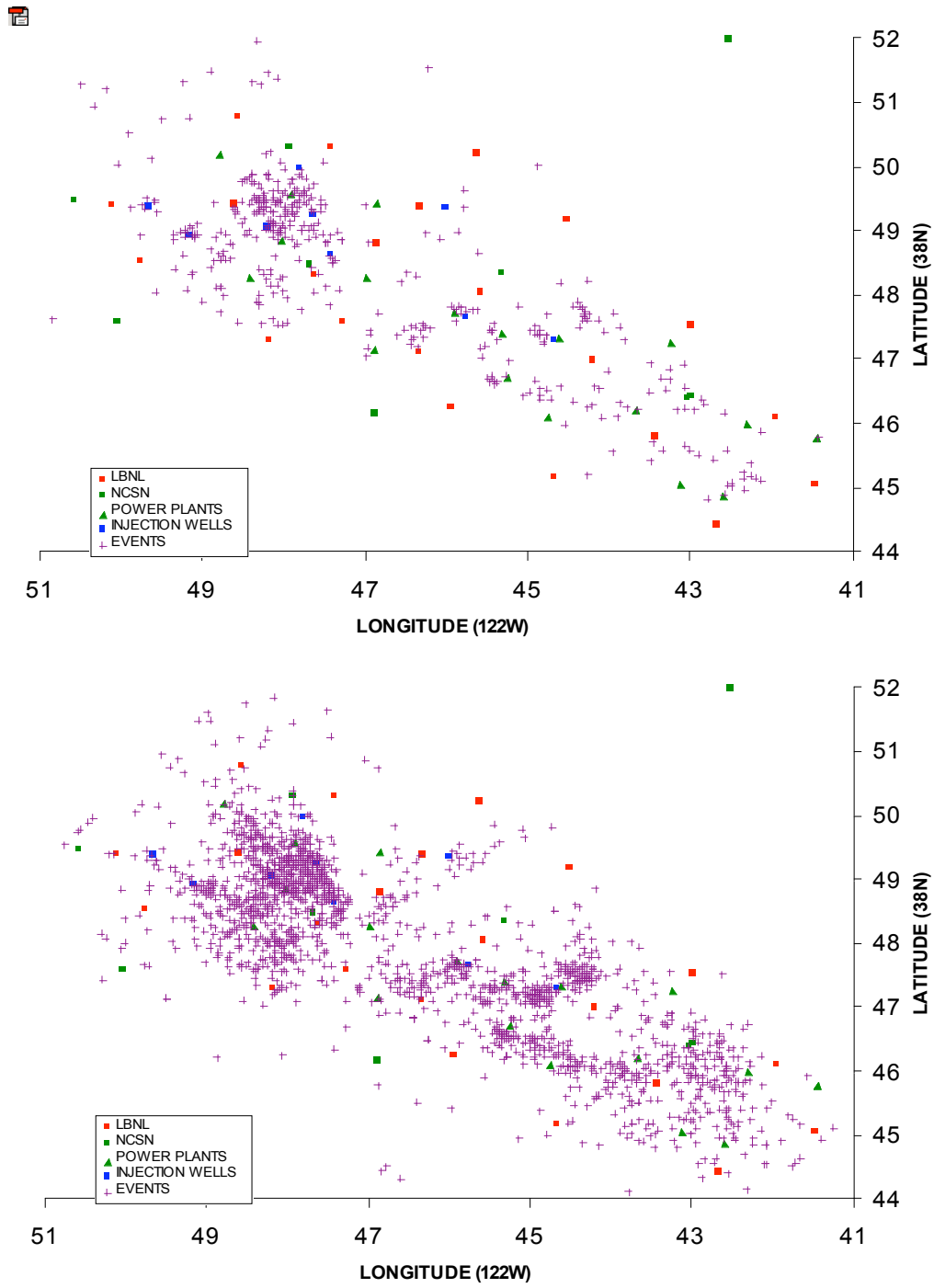
Figure 4. One month (April 2004) of data from the USGS array (top) and the LBNL array (bottom figure).
