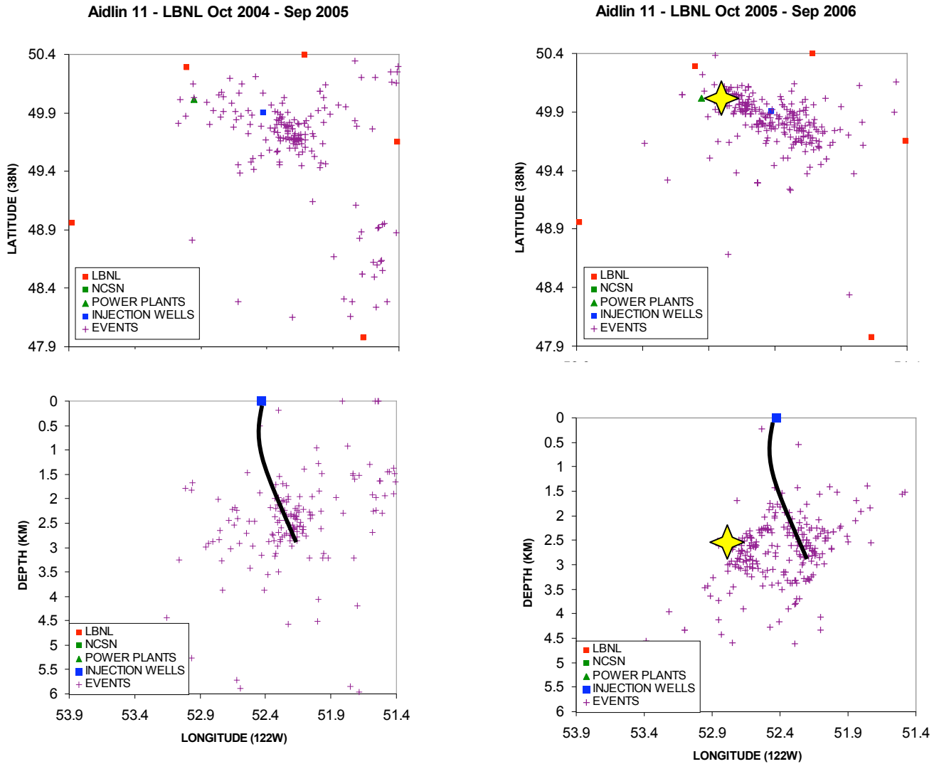
Figure 15. Location and depth of events in the Aidlin area of the Geysers. Also shown is the location of a magnitude 4 event in the vicinity that occurred in October of 2005.
