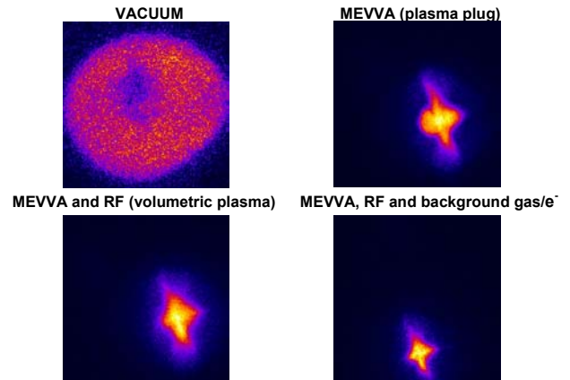
Figure 6: Spot size dependence on neutralization mechanism. Image box size is 4\text{cm} \times 4\text{cm} squares.
