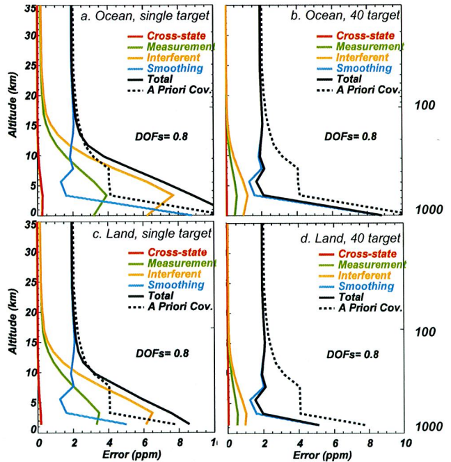
Fig. 1. Errors for an ocean scene (a,b) and land scene (c,d). Left panels show single target errors and right panels show errors for 40-target averages assuming a random distribution of measurement, interferent, and cross-state errors.
