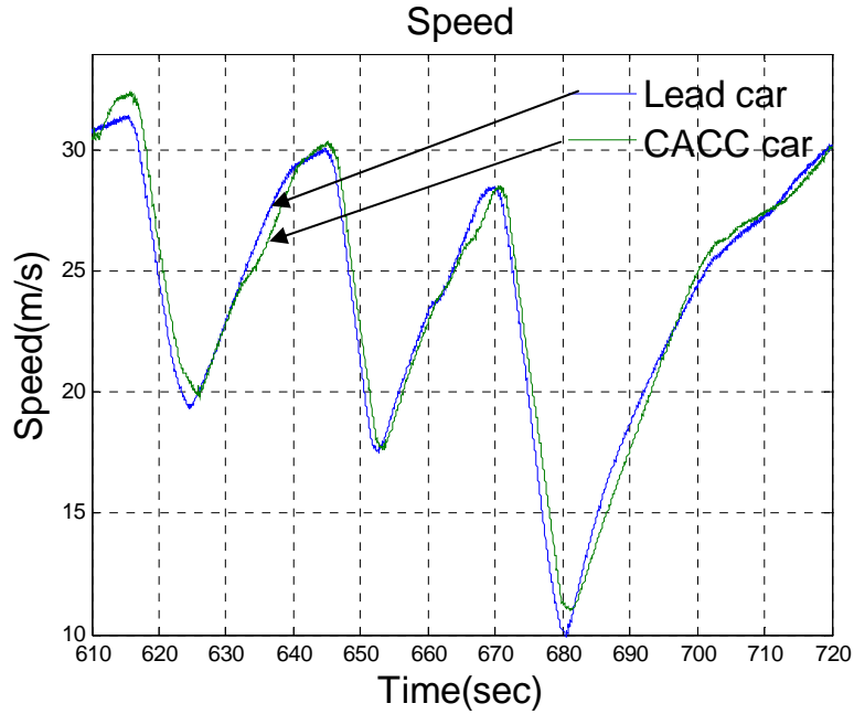
Figure 17: Speed profiles when leading car brakes and accelerates repeatedly
