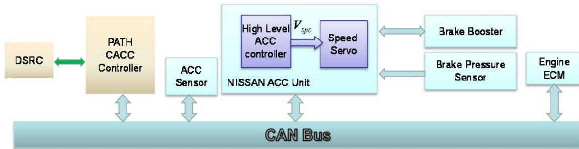
Figure 4: Add-on System Design for PATH CACC
