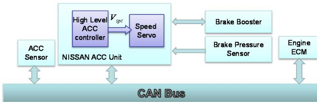
Figure 3: Configuration of Existing Nissan ACC Controller
