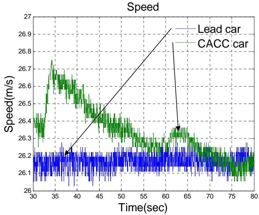
Figure 10: Proving ground test: steady state speed performance
