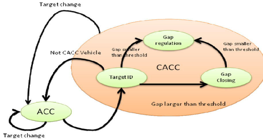
Figure 5: State Machine for PATH CACC controller
