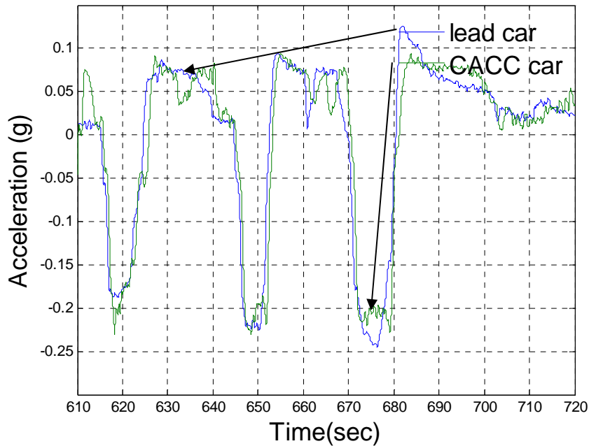
Figure 19: Acceleration profiles when leading car brakes and accelerates repeatedly
