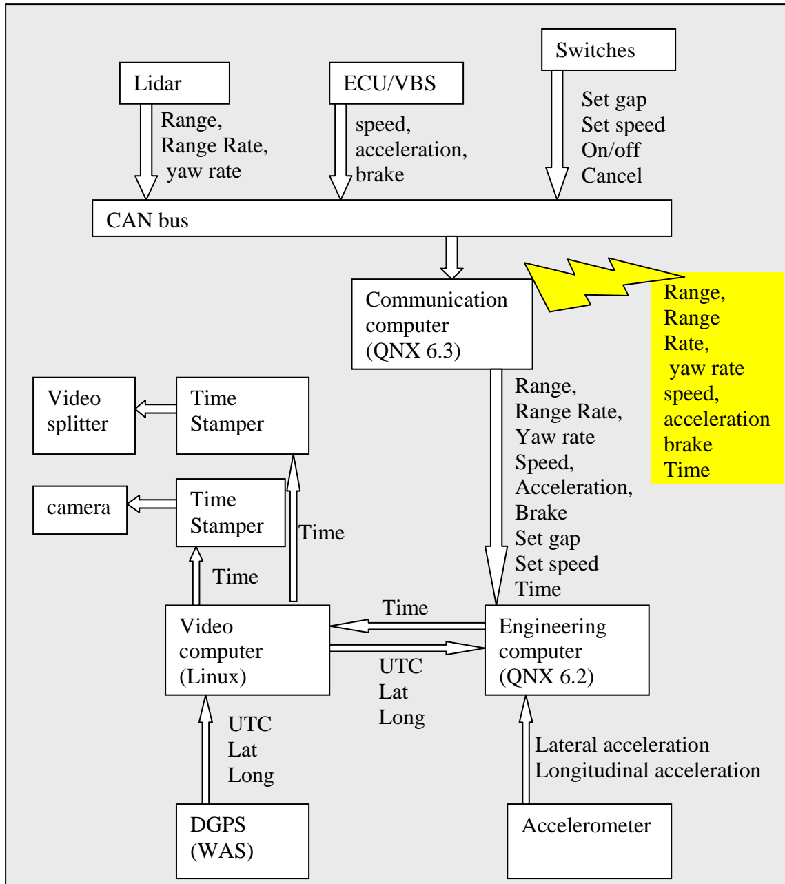
Figure 33: DAS Data Flow for Silver FX45 (ACC or lead vehicle for CACC)
