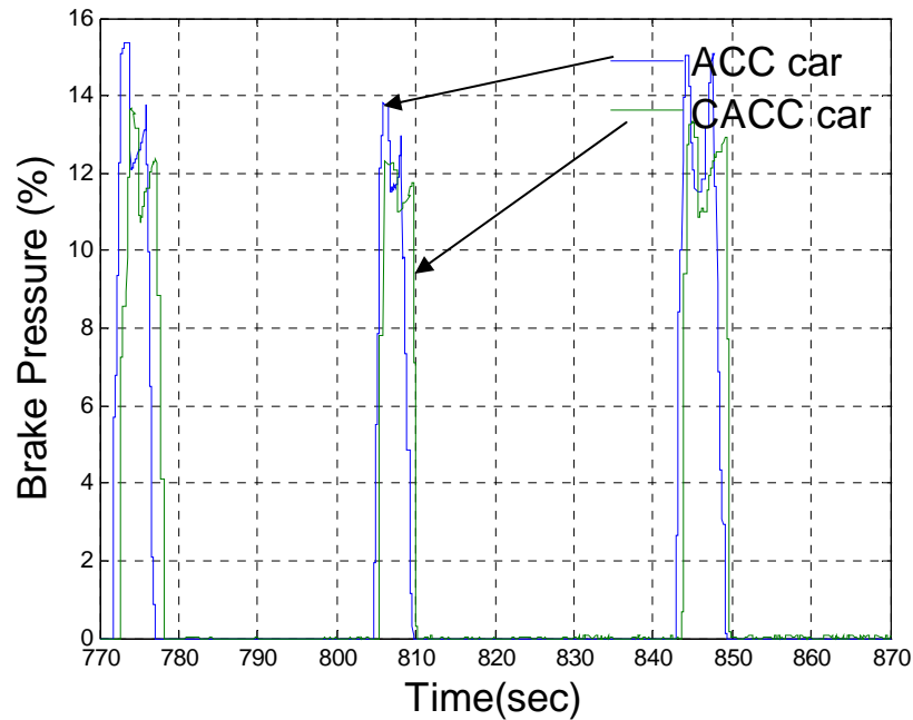
Figure 24: Three car platoon test – brake pressure
