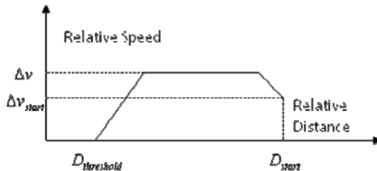
Figure 9: Trajectory Planning for CACC Gap Closing Controller
