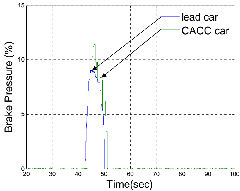
Figure 16: Brake pressure response when leading car brakes while CACC car is approaching
