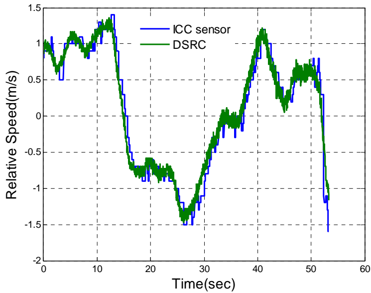
Figure 6: Comparison of relative speed output between ACC sensor and DSRC
