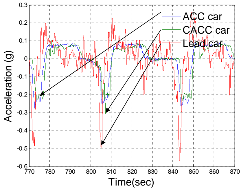
Figure 23: Three car platoon test - accelerations
