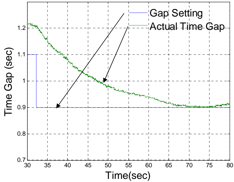
Figure 11: Proving Ground Test: steady state time gap performance
