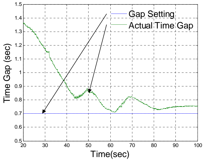
Figure 14: Time gap response when leading car brakes while CACC car is approaching
