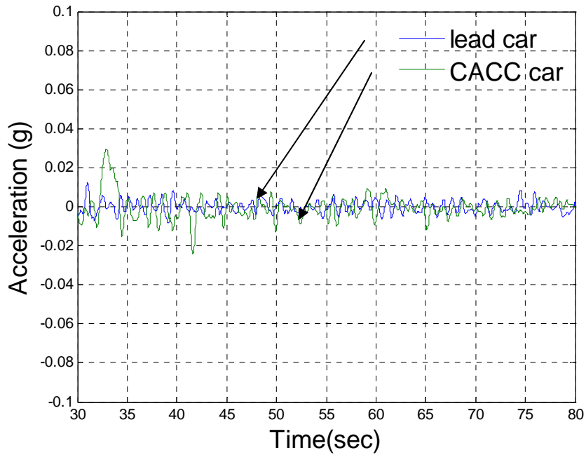
Figure 12: Proving Ground Test: steady state acceleration performance
