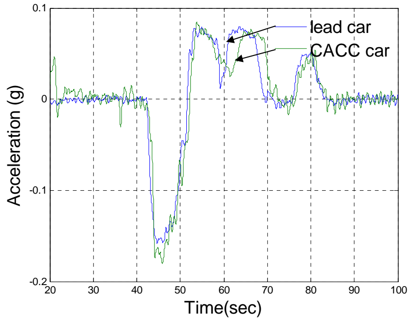
Figure 15: Acceleration response when leading car brakes while CACC car is approaching
