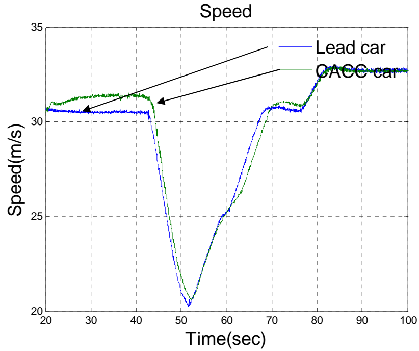
Figure 13: Speed response when leading car brakes while CACC car is approaching
