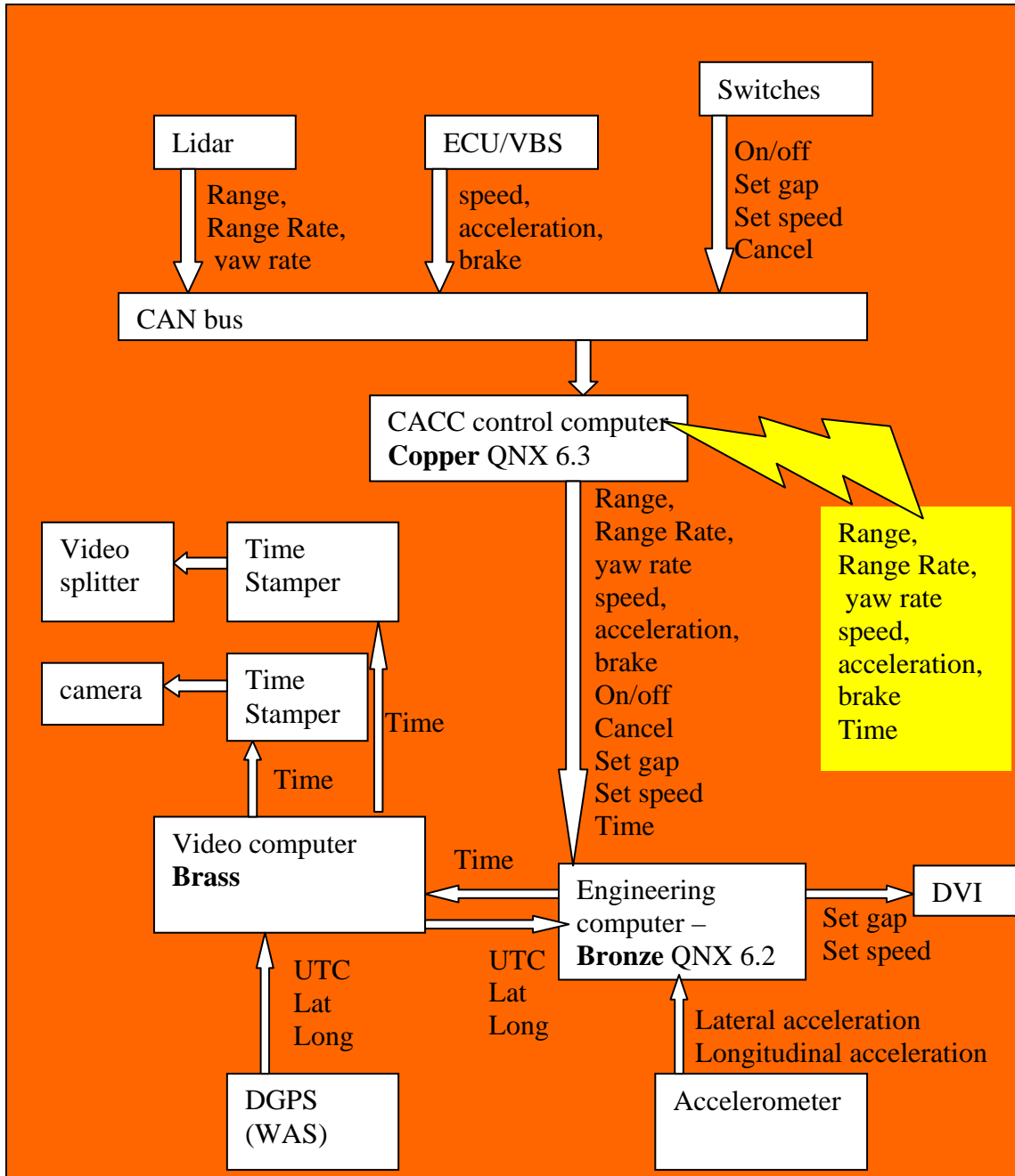
Figure 34: DAS Data flow for Copper (CACC) Vehicle
