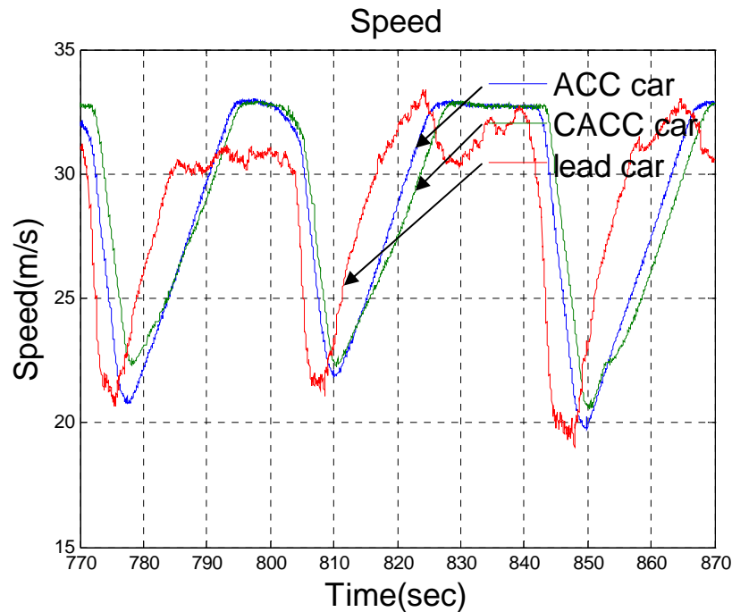
Figure 21: Three car platoon test – speed profiles
