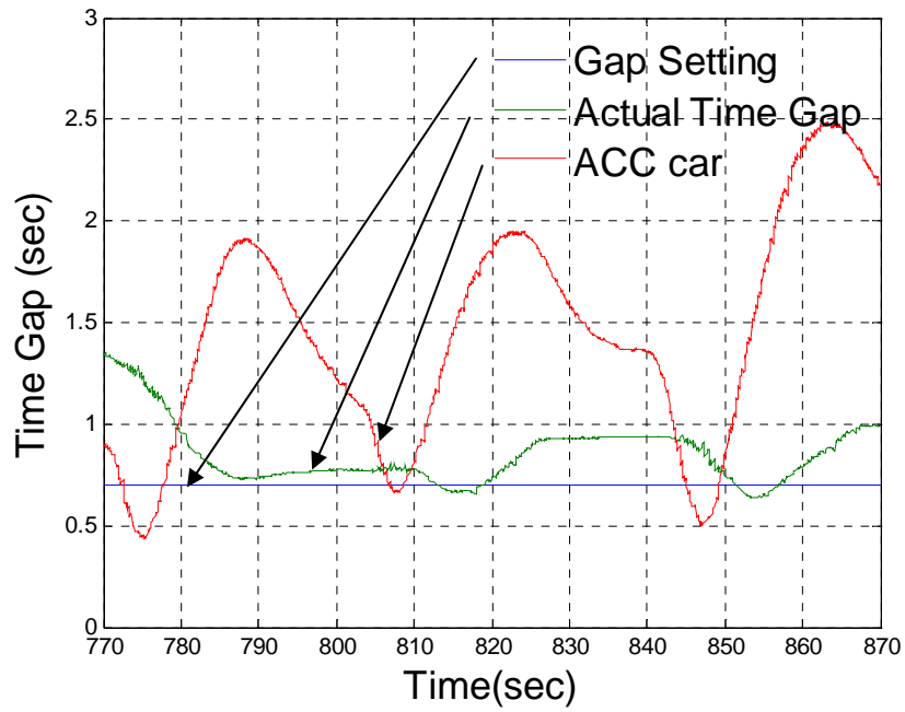
Figure 22: Three car platoon test – time gaps
