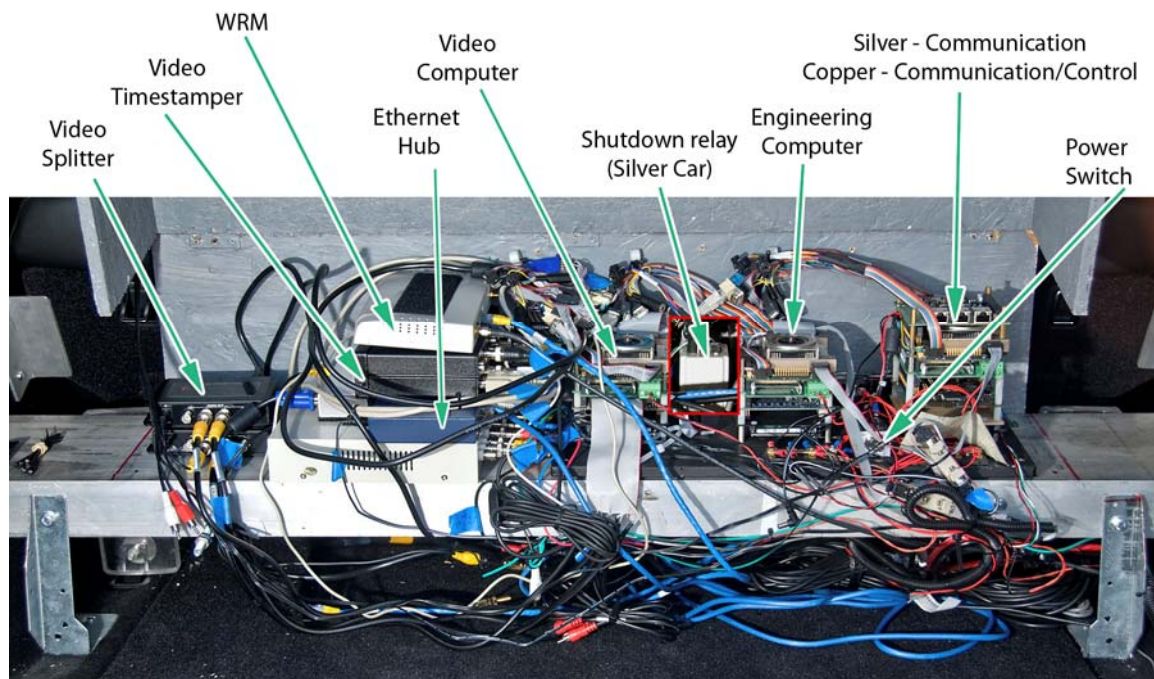
Figure 29: C/ACC DAS and Engineering Computer
