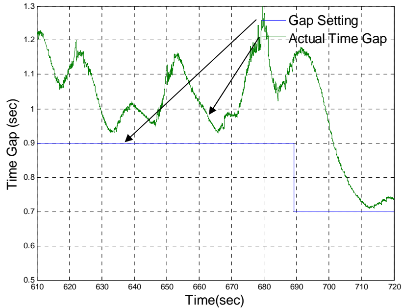
Figure 18: Time gap profiles when leading car brakes and accelerates repeatedly
