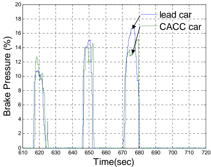
Figure 20: Brake pressure profiles when leading car brakes and accelerates repeatedly
