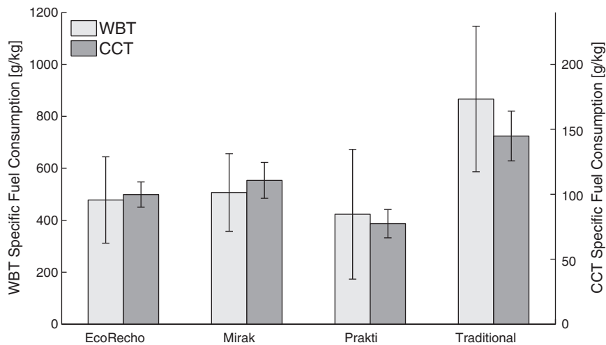
Fig. 8. Average specific fuel consumption [g/kg] during the WBTs and the CCTs. All improved stoves saved fuel compared to the traditional for both the WBTs (on average) and the CCTs (statistically significantly). Error bars represent 95% confidence intervals.
