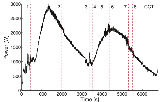
Fig. 12. Typical power cycle for a CCT of the traditional stove. Vertical numbered lines represent transitions in the test: 1. Bean Pot on; 2. Bean Pot simmering begins; 3. End Bean phase; 4. Vegetable Pot on; 5. Vegetable Pot off; 6. Bean Pot on again; 7. Rice added; 8. Rice and bean mixture simmering begins.
