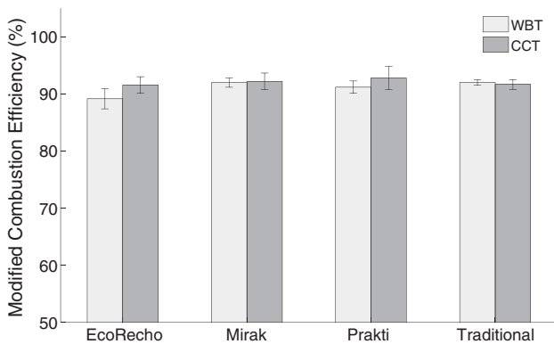
Fig. 10. The modified combustion efficiency for both the WBTs and CCTs; error bars represent 95% confidence intervals. Overall, the MCEs are comparable across the stoves, with a deviation between stoves of less than 3.3% for the WBTs and 0.6% for the CCTs. The values range from 89% to 93% indicating smoldering to mixed combustion, which is as expected for charcoal combustion.
