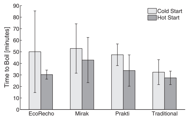
Fig. 6. The time to boil 2.5 L of water, reported in minutes, for both cold and hot starts. For cold starts, the traditional stove was noticeably faster on average than any other stove, but for hot starts, the EcoRecho and Prakti stoves were similar to the traditional one. Error bars represent 95% confidence intervals.
