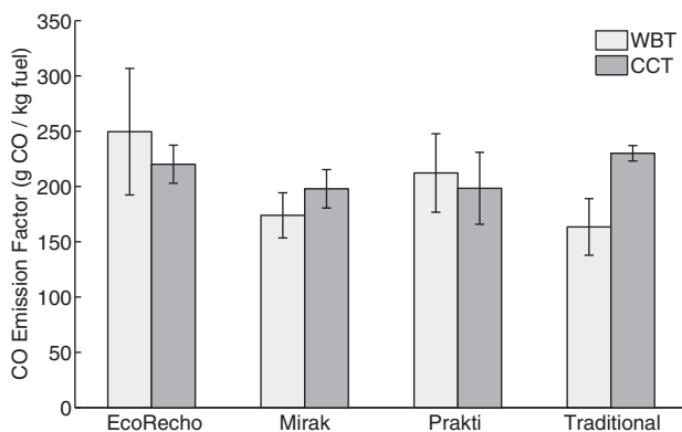
Fig. 9. The CO emission factors [g CO/kg fuel dry consumed] for each stove. For the WBTs, the Mirak and traditional stoves had lower emission factors, while for the CCTs, the Mirak and Prakti stoves had lower values. However, it is important to note that the traditional stove uses more fuel than the others to complete each test and emits more CO. Error bars represent 95% confidence intervals.
