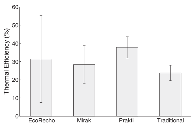
Fig. 7. Average thermal efficiency for the WBTs. All improved stoves had on average a higher thermal efficiency than the traditional one with the Prakti stove having a statistically significantly better thermal efficiency ( p = 0.05 ). Error bars represent 95% confidence intervals.
