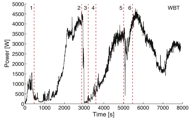
Fig. 11. Typical power cycle for a WBT of the traditional stove. Vertical numbered lines represent transitions in the test: 1. Pot on for the cold start; 2. End cold start; 3. Begin hot start; 4. Pot on for the hot start; 5. End hot start; 6. Begin simmer.
