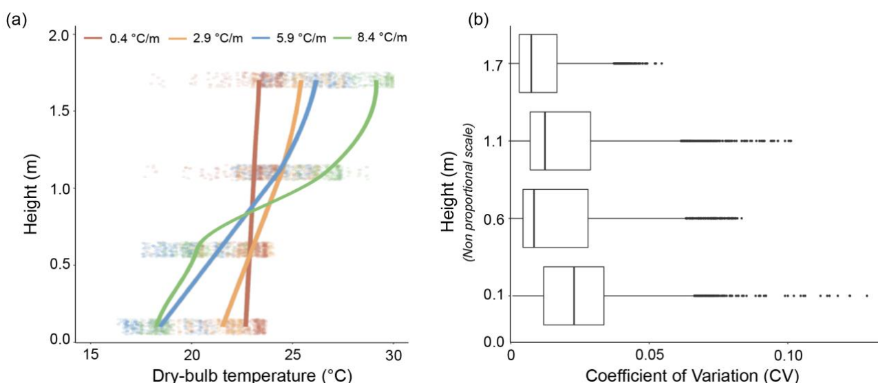
Figure 2. Air temperatures and measurement variations at 0.1, 0.6, 1.1, and 1.7 m; a) Dry-bulb temperature. A curve is the local polynomial regression (LOESS) fit of the raw data points (scattered in the plot) at each corresponding vertical temperature gradient; b) Coefficient of variation (standard deviation divided by mean) of temperatures measured at three locations in Figure 1.
