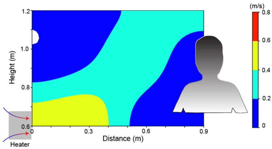
Figure A1. Mid-plane air speed distribution in front of a fan heater (1500 W) that was placed 0.6 m above the floor and 0.8-1.0 m away from a subject. The air speed was tested at the maximum fan setting, higher than the conditions in the experiment. The ambient temperature for the air speed measurement was 23.3 °C.
