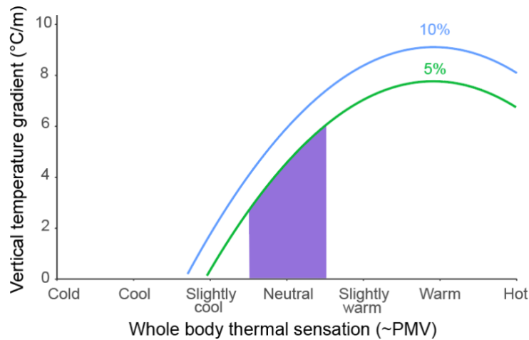
Figure 9. Allowed vertical temperature gradient between head (1.1 m) and feet (0.1 m) for local discomfort. The shaded area denotes the allowed vertical temperature gradient for 5% dissatisfied when thermal sensation is designed from -0.5 to 0.5.
