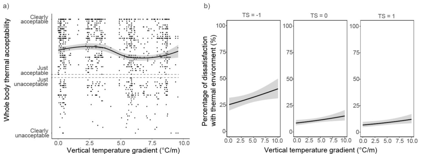
Figure 6. Whole-body thermal acceptability and the percentage dissatisfied with the thermal environment at different vertical temperature gradients between head and feet. a) Whole-body thermal acceptability ( n = 1177 ); b) The predicted percentage of dissatisfaction with the thermal environment at three thermal sensations ( TS = -1, 0, 1 ) using logistic regression, Equation 1 (The grey shades represent pointwise 95% confidence interval for the fitted values).
