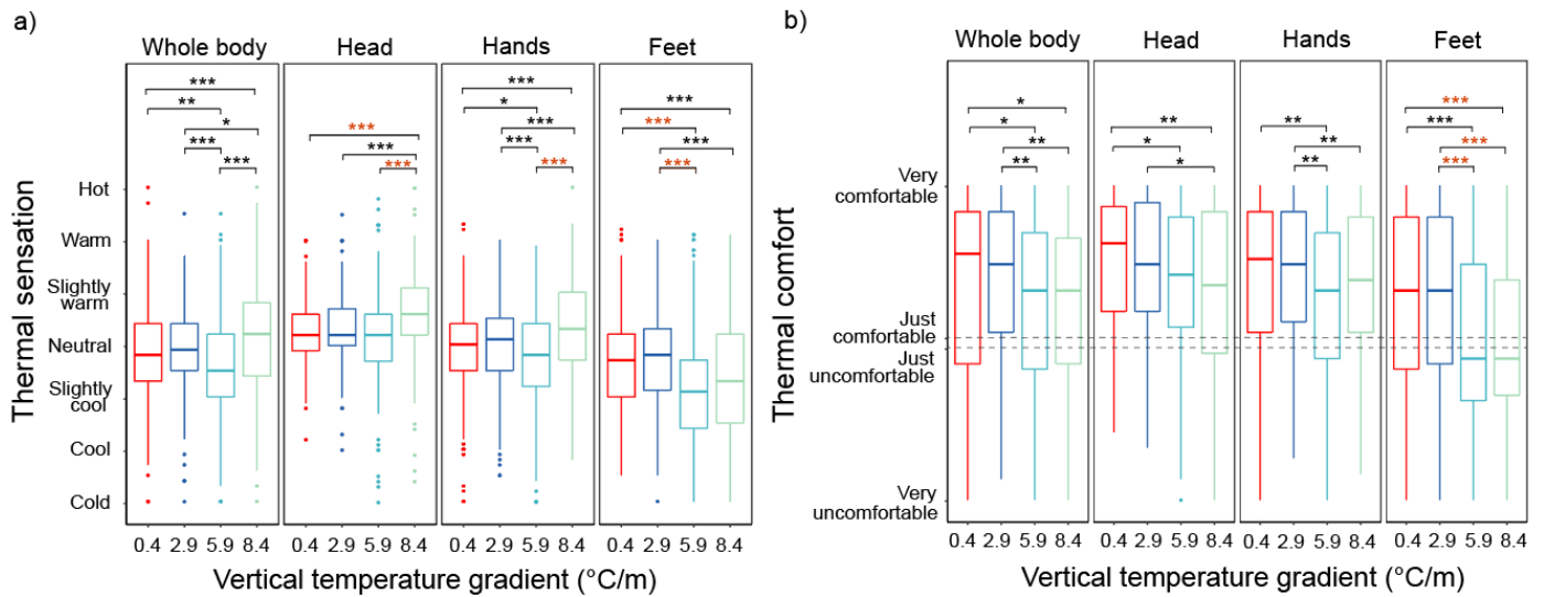
Figure 4. Thermal sensation and thermal comfort varying with vertical temperature gradient; a) whole-body and local thermal sensation; b) whole-body and local thermal comfort. (Statistical significance: * p < 0.05 , ** p < 0.01 , and *** p < 0.001 ; Stars in red refer to medium or higher effect sizes based on Cohen's d ; |d| < 0.147 "negligible", |d| < 0.33 "small", |d| < 0.474 "medium", otherwise "large")
