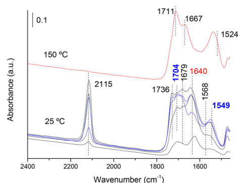
Figure 1. Temperature-programmed FT-IR spectra of 1 adsorbed on Au-TiO 2 at increasing dosing (black lines), after evacuation at 10 -6 mbar (blue lines) at 25 °C, and after increasing temperature to 150 °C (red line).
