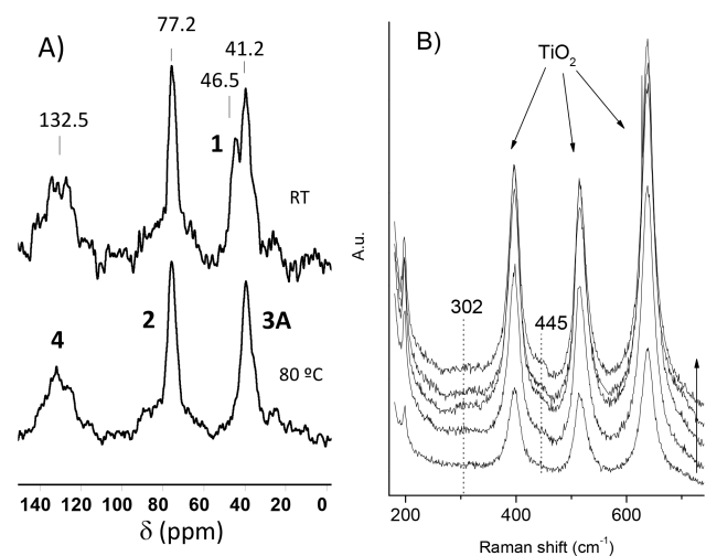
Figure 2. (A) ^{13}\text{C} CP/MAS NMR spectra of Au–TiO 2 loaded with 1 (Au/1 = 5) at RT (top) and after heating at 80 °C for 30 min (bottom). Spectrometer frequency is 100.6 MHz and spinning rate is 5 kHz. (B) Raman spectra of 1 adsorbed on Au–TiO 2 at RT and evolution with time (24, 35, 46, 74, and 86 min).
