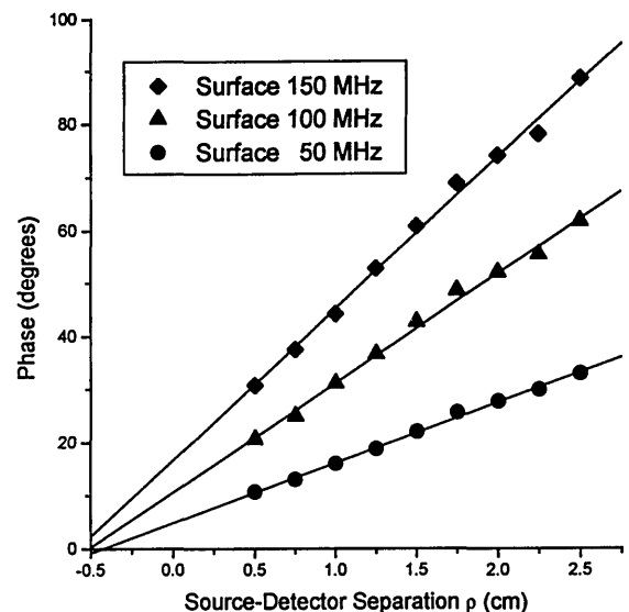
Fig. 9. Phase versus fiber separation for three different modulation frequencies: 50, 100, and 150 MHz. The source and the detector fibers were either pushed deep into the gel to simulate an infinite-medium geometry (A) or placed on the surface of the gel (B). The gel was the same one used in Figs. 6–8. For both infinite-medium and surface data the x intercepts are approximately -0.5 cm.
