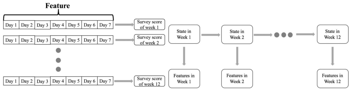
Fig. 3. Illustration of independent week model (left) and Hidden Markov Model (right). For HMM, feature in each week was observed while the state of health status transits from week to week.
