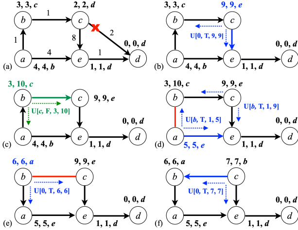
Figure 1: Fast convergence without blocking in SCRIP
