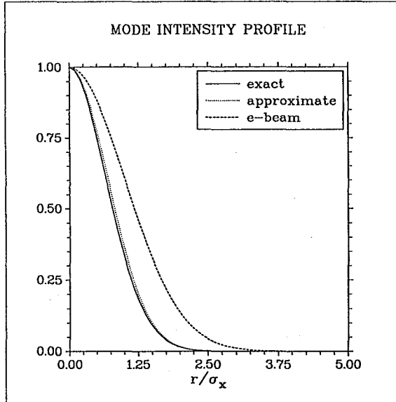
FIG. 1. Intensity profile of E_{00} mode from exact solution and variational approximation, superimposed with electron density profile.
