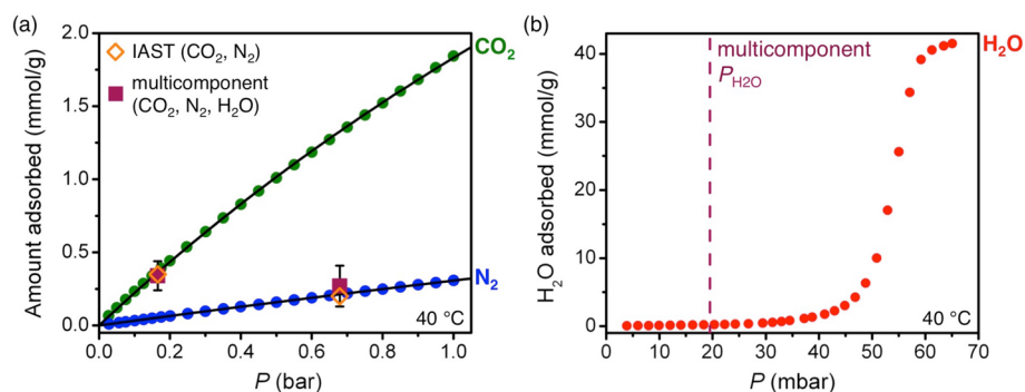
Figure 6. (a) Circles represent single-component \text{CO}_2 (green) and \text{N}_2 (blue) adsorption isotherms at 40^\circ\text{C} for the activated carbon AX-21. Black lines correspond to single-site Langmuir fits. Square data points represent the amount of \text{CO}_2 and \text{N}_2 adsorbed from a mixture of \text{CO}_2 (166 mbar), \text{N}_2 (679 mbar), and \text{H}_2\text{O} (20 mbar) at 40^\circ\text{C} . Orange diamonds represent the amount of \text{CO}_2 and \text{N}_2 predicted to be adsorbed by IAST from a mixture of \text{CO}_2 (166 mbar) and \text{N}_2 (679 mbar). (b) Pure \text{H}_2\text{O} adsorption isotherm (red circles) for AX-21 at 40^\circ\text{C} . The purple dashed line represents the partial pressure of \text{H}_2\text{O} in the multicomponent experiment.
