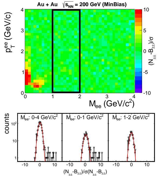
FIG. 12. (Color online) Upper panel: Residual differences between same-event and mixed-events like-sign distributions divided by its standard deviation. The black box indicates the default normalization region. Bottom panel: Residual difference distributions for all the entries in different mass regions.
