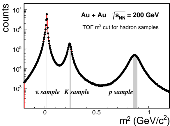
FIG. 5. Charged particle m^2 distribution from TOF measurements in 200 GeV Au+Au minimum bias collisions. The shaded areas are the respective m^2 thresholds used for selecting high purity \pi , K , p samples.
