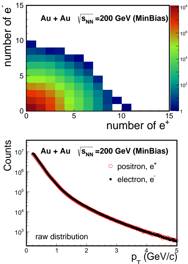
FIG. 4. Upper panel: The distributions of number of electron candidates. Bottom panel: Raw p_T spectra of the electron candidates.
