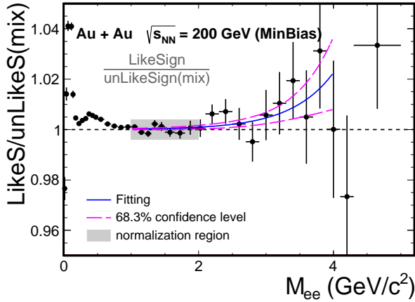
FIG. 18. Ratio of the same-event like-sign to the mixed-event unlike-sign distributions. The gray area indicates the normalization region. The solid and dashed lines depict an empirical fit to the distribution in the mass region of 1–4 GeV/ c^2 and the fit uncertainties, respectively.
