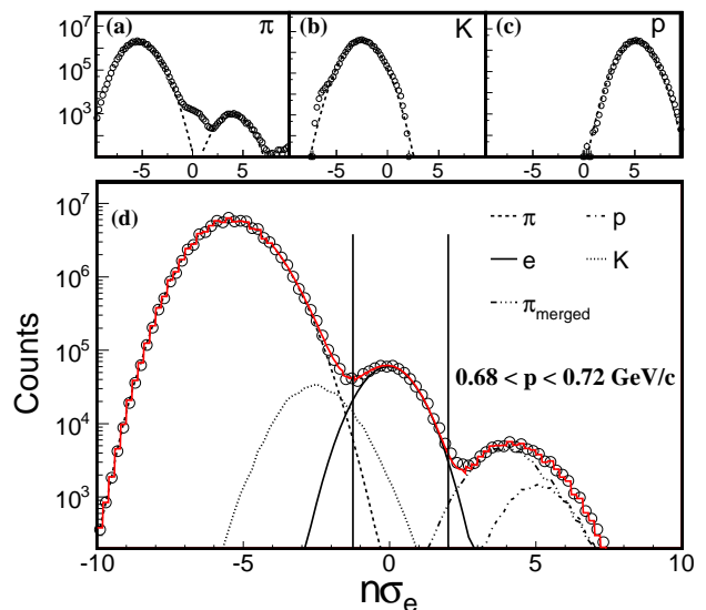
FIG. 6. Upper panel: n\sigma_e distribution of clean \pi , K , p samples selected using TOF masses. Dashed lines are Gaussian fits to these distributions allowing the extrapolation of the tail regions where contamination becomes apparent. Bottom panel: An example of multi-component fit to the n\sigma_e distribution for the momentum bin 0.68 < p < 0.72 GeV/ c in 200 GeV Au+Au minimum bias collisions. The two vertical lines indicate the selected electron range.
