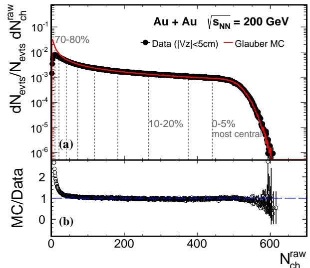
FIG. 1. Upper panel: Uncorrected multiplicity N_{\text{ch}}^{\text{raw}} distribution measured within |\eta| < 0.5 and |V_z| < 5 cm. The solid curve depicts the multiplicity distribution from a MC Glauber simulation. Bottom panel: Ratio between MC and data.
