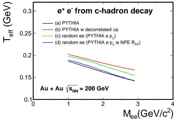
FIG. 38. (Color Online) Slope parameters T_{\text{eff}} versus invariant mass for dielectrons from charm hadron decays. Different lines show the outcome from PYTHIA calculations assuming different levels of correlations between charm pairs.
