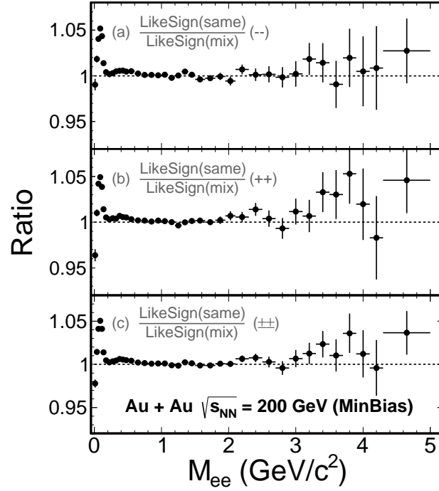
FIG. 14. Panel (a), (b), (c): Ratios between same event and mixed-event like-sign distributions.
