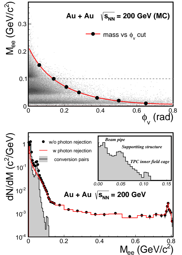
FIG. 9. Upper panel: \phi_V vs. mass distributions for photon conversion electron pairs from the full GEANT MC simulation. The solid red line depicts the mass dependent \phi_V cut that was used to remove these conversion pairs. Bottom panel: photon conversion contribution in 200 GeV Au+Au minimum bias collisions. The insert plot shows the structures from the beam pipe, the supporting bars of the inner cone, and the TPC inner field cage.
