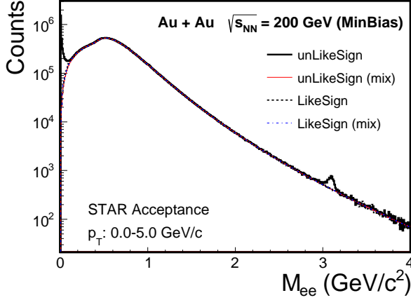
FIG. 13. (Color online) Raw pair mass distributions for 200 GeV Au + Au collisions. The mixed-event unlike-sign and like-sign distributions are normalized in the mass region from 1.0 to 2.0 GeV/c 2 .
