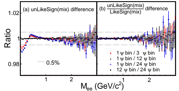
FIG. 10. (Color online) Difference in mixed-event distributions when using different number of event pools in the reconstructed event-plane angle. The left plot shows differences of unlike-sign distributions with different divisions and the right plot shows differences of ratios of unlike-sign to like-sign distributions.
