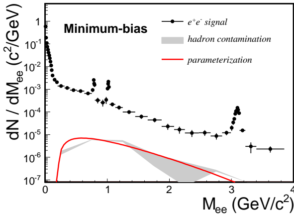
FIG. 26. Estimated hadron contamination from e-h and h-h contributions due to the finite contaminated hadrons in the electron sample compare to the e^+e^- pair signal in 200 GeV Au+Au collisions.
