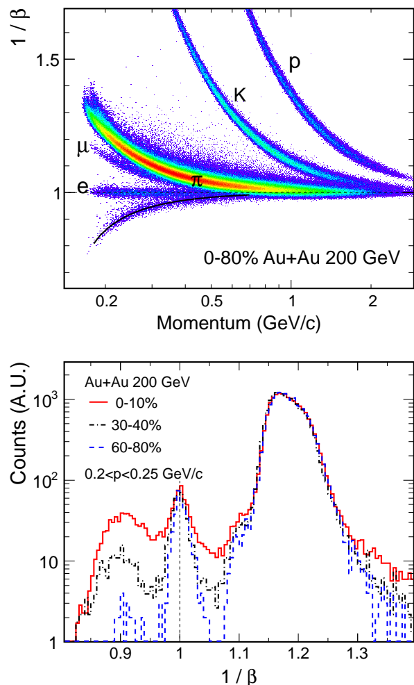
FIG. 3. (Color online) Upper panel: 1/\beta vs. particle momentum. Solid line depicts a prediction for those associations where TOF hits were triggered by conversion electrons while matched randomly with TPC charged tracks. Bottom panel: 1/\beta projection in the momentum bin 0.2 < p < 0.25 GeV/c for three centrality bins, normalized to the pion peak region.
