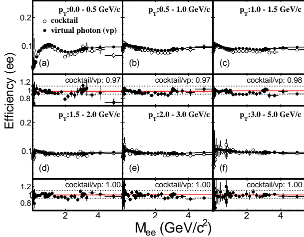
FIG. 22. e^+e^- pair efficiency as a function of pair mass in different p_T regions calculated from two different methods.
