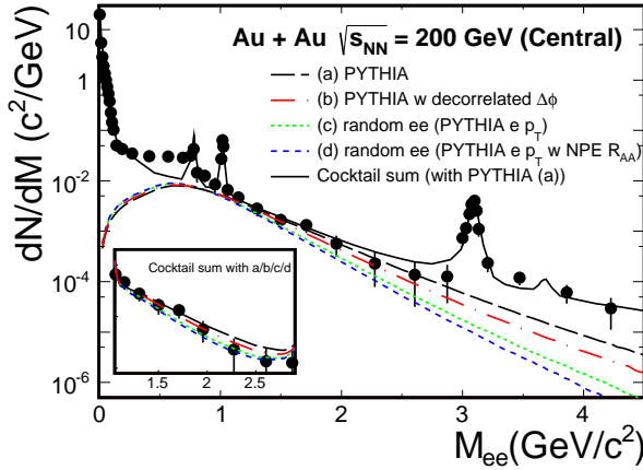
FIG. 37. (Color Online) Correlated charm contributions to the dielectron mass spectra for different assumptions of the correlation strength. The simulations are compared to the measured dielectron spectrum in the most central (0-10%) Au+Au collisions. The total cocktail shown is calculated using the default PYTHIA correlations. The insert plot shows the comparison between the cocktail sums with above four different charm contributions and the measured spectrum in the IMR.
