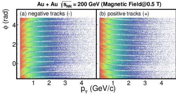
FIG. 16. (Color online) \phi vs. p_T for all negative (left panel) and positive (right panel) tracks from a single magnetic field configuration. The blank areas are due to the TPC sector boundaries, which shows the different acceptances between positive and negative tracks particularly in the low p_T due to the magnetic field.
