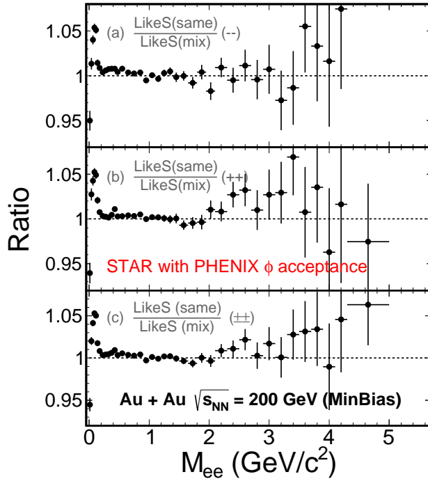
FIG. 45. Ratios of pair distributions for electron candidates selected with the PHENIX \phi acceptance. Panels (a), (b), (c): ratios of like-sign distributions between same event and mixed-event.
