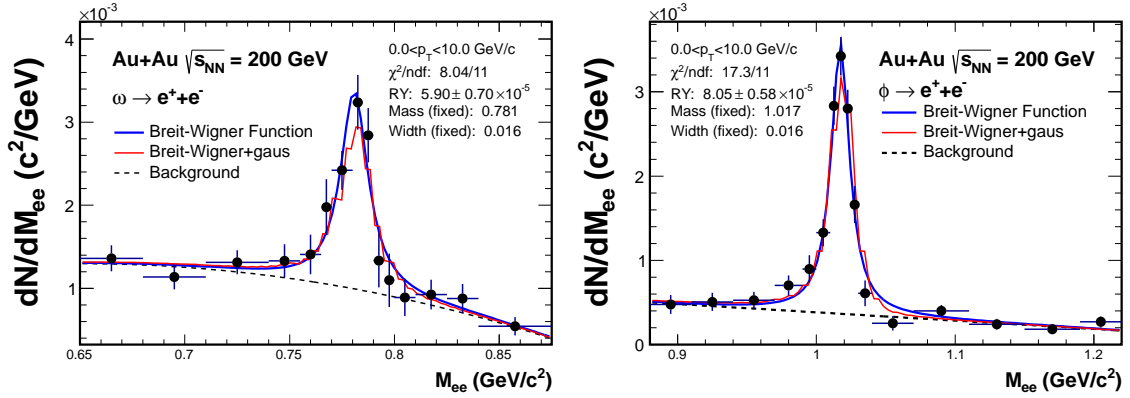
FIG. 39. (Color Online) \omega and \phi meson invariant mass distribution from \sqrt{s_{NN}} = 200 GeV Au+Au minimum-bias collisions after subtraction of the combinatorial background using the mixed-event method. The blue and red lines depict two functions used for the signals in the fit. A second-order polynomial function is used to describe the residual correlated background.
