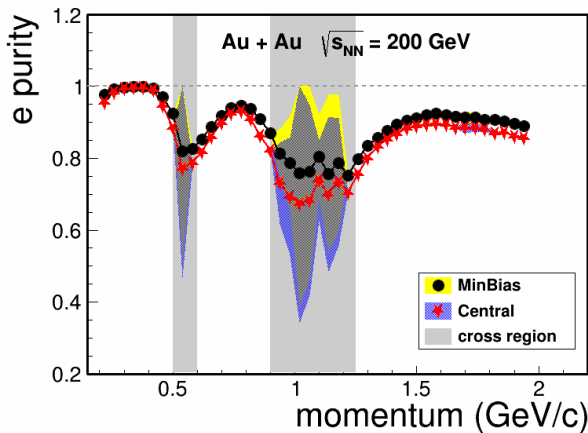
FIG. 7. (Color online) Estimated electron purity vs. momentum in 200 GeV Au + Au collisions. Gray areas indicate the momentum regions where n\sigma_e of kaons and protons cross with that of electrons resulting in large uncertainties in those ranges.
