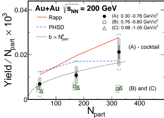
FIG. 36. (Color Online) The yields scaled by N_{\text{part}} for the \rho -like region with the cocktail subtracted, and the \omega -like and the \phi -like regions without cocktail subtraction as a function of N_{\text{part}} . Model calculations are included as red solid and dot-dashed curves, while the dashed curve depicts a power-law fit to the yield/ N_{\text{part}} for the \rho -like region with the cocktail subtracted. Systematic uncertainties from the data are shown as grey boxes, and the green brackets depict the total systematic uncertainties including those from cocktails. For clarity, the \omega -like and \phi -like data points are slightly horizontally displaced.
