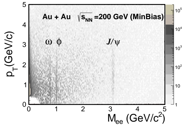
FIG. 8. Two-dimensional ( M_{ee}, p_T ) distribution of unlike-sign e^+e^- pairs with background subtraction from 200 GeV Au + Au minimum bias collisions in the STAR acceptance ( p_T > 0.2 \text{ GeV}/c , |\eta| < 1 , and |y_{ee}| < 1 ).
