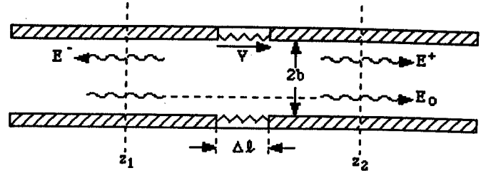
Fig. 3 Geometry for analysis of radiated TM waves
