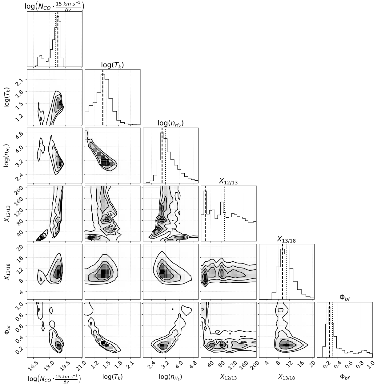
Figure 2.6. Marginalized 1D and 2D likelihood distributions of a faint pixel at (R.A., Decl.) = (10^{\text{h}}43^{\text{m}}57^{\text{s}}.8, 11^{\circ}42'15''.5) in the gap region between the ring and the nucleus. See the caption of Figure 2.5 for more information.
