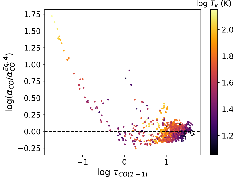
Figure 3.16. Ratio of the modeled and fitting-predicted \alpha_{\text{CO}} (by Equation 3.4) versus the CO optical depth, color-coded by the modeled gas temperature. The dashed line indicates perfect agreement between the modeled and predicted \alpha_{\text{CO}} . The fitted Equation 3.4 should be limited to optically thick regions, where the 25–75th percentile scatter along the y-axis is 0.12 dex.
