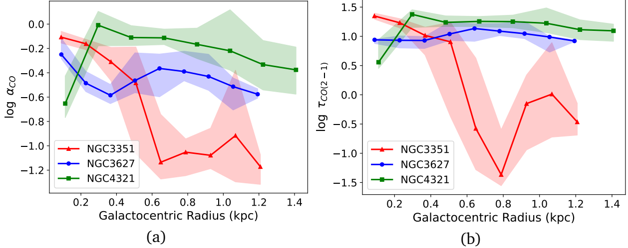
Figure 3.13. Medians of the modeled (a) \alpha_{\text{CO}} in units of M_{\odot} (\text{K km s}^{-1} \text{pc}^2)^{-1} and (b) line center \tau_{\text{CO}(2-1)} within \sim 100 pc galactocentric radii bins in the centers of NGC 3351 (red), NGC 3627 (blue), and NGC 4321 (green). Shaded areas span the 25th and 75th percentile ranges. All regions show \alpha_{\text{CO}} at least a factor of four lower than the Galactic value of \log(\alpha_{\text{CO}}) = 0.64 . The radial trend of \alpha_{\text{CO}} is mostly consistent with that of \tau_{\text{CO}(2-1)} in all three galaxy centers except in NGC 3627’s nucleus.
