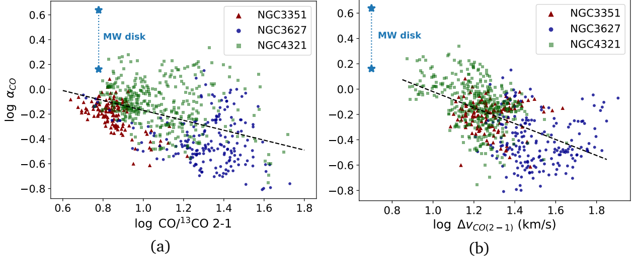
Figure 3.17. Relation of the modeled \log(\alpha_{\text{CO}}) with the observed (a) CO/ ^{13}\text{CO} 2–1 line ratio and (b) CO 2–1 effective line width in optically thick regions with \tau_{\text{CO}(2-1)} > 5 . The dashed lines represent the best-fit power law relations (Equations 3.5 and 3.6). The typical Milky Way disk values with x_{\text{CO}} ranging from \sim 10^{-4} (higher \alpha_{\text{CO}} ) to 3 \times 10^{-4} (lower \alpha_{\text{CO}} ) are labeled by the blue stars. The data points cover all regions except the inflow regions of NGC 3351. Despite a \sim 0.4 dex scatter in both relations, there is a clear trend of \alpha_{\text{CO}} decreasing with the line ratio and CO line width, suggesting these observable properties as potential tracers for \alpha_{\text{CO}} variations in galaxy centers.
