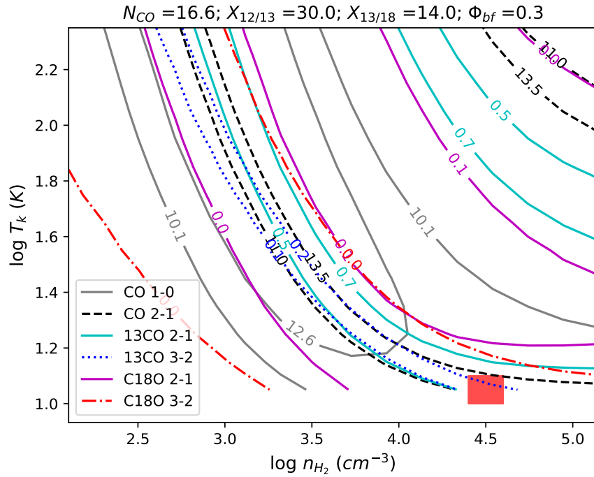
Figure 2.14. Constraints on the T_k – n_{H_2} slice where the best-fit parameter (red box) lies assuming a 10% flux uncertainty. See the caption of Figure 2.7 for more information.
