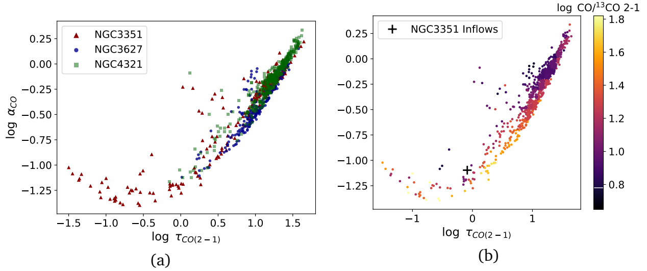
Figure 3.14. Modeled \alpha_{\text{CO}} and \tau_{\text{CO}(2-1)} , color-coded by (a) three galaxies and (b) 2D-binned medians of the observed \text{CO}/^{13}\text{CO} 2–1 ratios. In panel (b), the black cross sign represents spectral stacking result of the NGC 3351 inflows (see Teng et al. 2022 and Appendix 3.B), and the white line on the color bar indicates the typical ratio found in the disks of Milky Way or other nearby galaxies. In the optically thick regime ( \tau_{\text{CO}} > 1 ), a positive correlation of \alpha_{\text{CO}} with \tau_{\text{CO}} is constantly seen in the three galaxy centers, and the \text{CO}/^{13}\text{CO} 2–1 ratio generally reflects the \tau_{\text{CO}} variation in optically thick regions.
