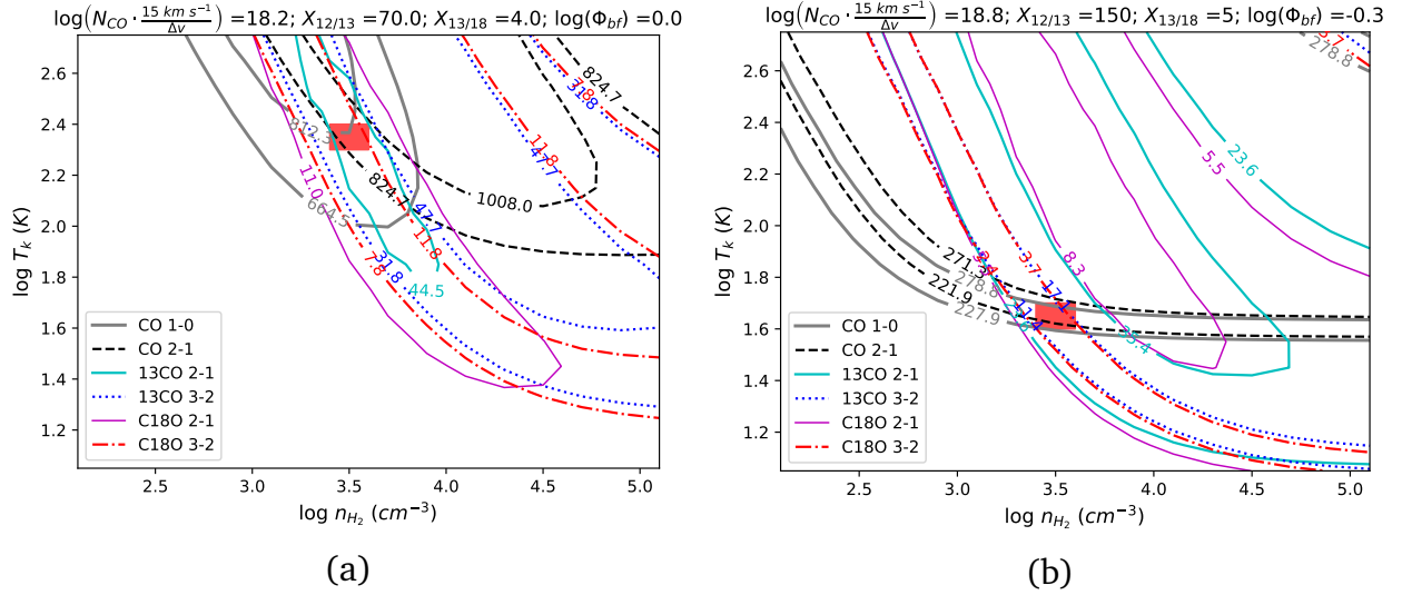
Figure 3.7. Best-fit (i.e. lowest \chi^2 ) constraints from the six observed line fluxes at (a) the central pixel and (b) a pixel in the northern, inner arm of NGC 4321. Contours show the ranges of observed line intensities \pm 1\sigma uncertainties, including the measurement and calibration uncertainties. Red boxes represent the best-fit solutions. Note that these are the solutions with the lowest \chi^2 value in the full grid, not the 1DMax solutions based on the marginalized PDFs, and thus the X_{12/13} values here may deviate from the lower X_{12/13} suggested by 1DMax solutions. Except for X_{12/13} , other parameters are similar to the 1DMax solutions as their 1D likelihoods are single-peaked and well-constrained (see Figure 3.8 and related discussion).
