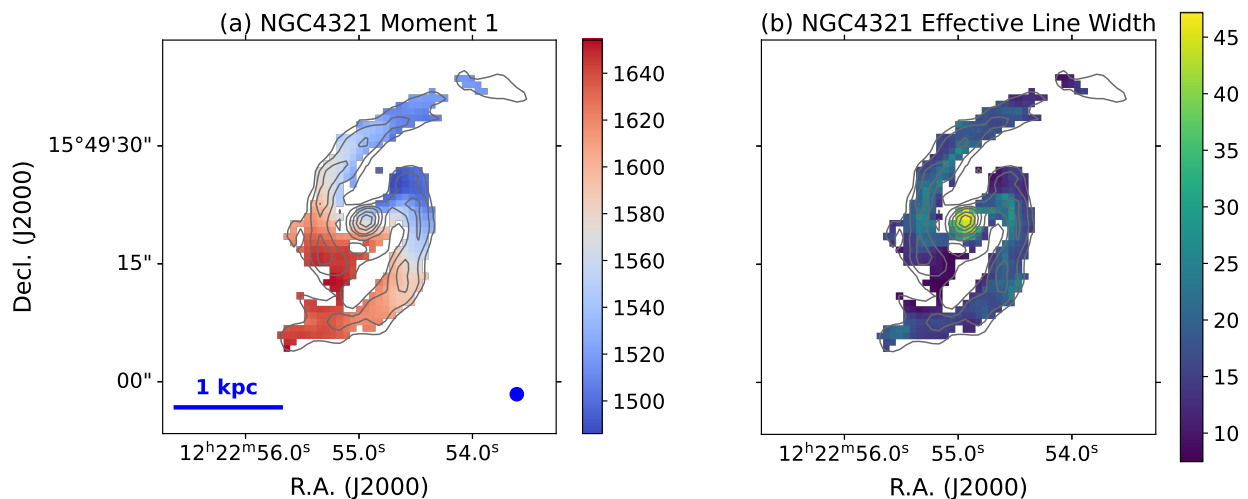
Figure 3.23. Maps of the CO 2–1 (a) moment 1 and (b) effective line width for NGC 4321, both in units of \text{km s}^{-1} .
