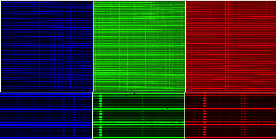
Figure 3. (top) A 2D spectrogram from the APOGEE instrument. The three chips (“blue”, “green”, and “red”) are shown with wavelength increasing to the right across the full APOGEE wavelength range of 1.514–1.696 \mu\text{m} . The gaps between the chips are slightly larger than as displayed in this image. Each fiber is imaged onto several pixels (vertically). Note the vertical series of points from sky lines in each fiber, and the horizontal spectra of faint stars and sky fibers. (bottom) Expanded view of the central 18 fibers and central 6 nm of each chip.
