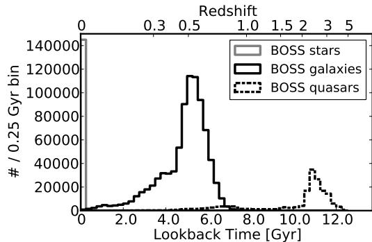
Figure 14. The distribution of BOSS DR10 spectroscopic objects versus lookback time for the 144,968 unique stars; 859,322 unique galaxies; and 166,300 unique quasars. Lookback time is based on the observed redshift under the assumption of a \Lambda CDM cosmology (Komatsu et al. 2011). This figure is nearly identical to the equivalent for DR9 (Figure 3 of Ahn et al. (2012)), scaled by a factor of 1.8.
