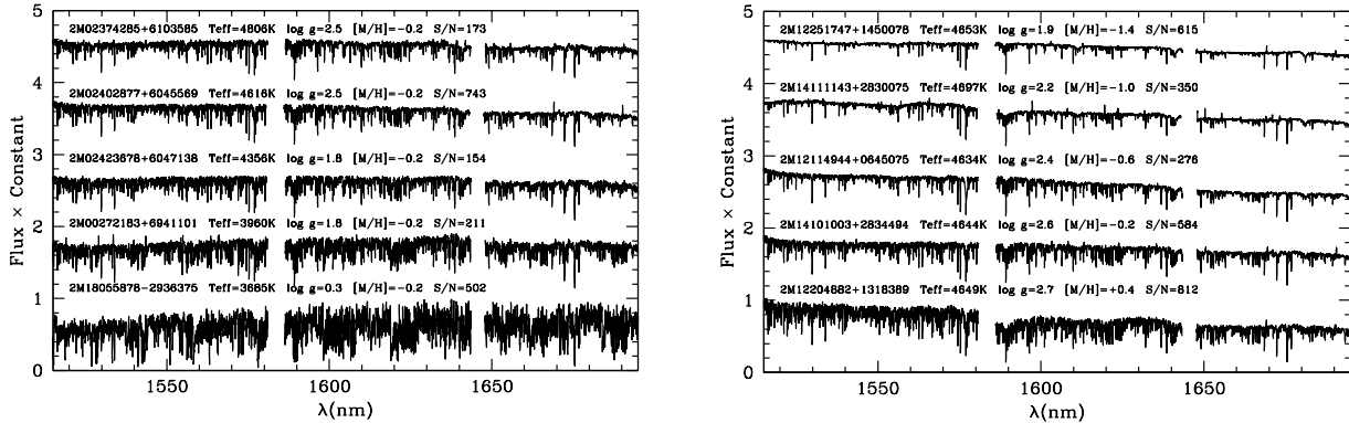
Figure 9. Typical APOGEE spectra at high S/N. (left) Spectra of stars with 5000 \text{ K} > T_{\text{eff}} > 3750 \text{ K} at constant [M/H] = -0.2 (a characteristic [M/H] for the sample). The trend in line intensity from top to bottom is driven by decreasing T_{\text{eff}} (which is strongly correlated with \log g – see Figure 11). (right) Spectra of stars with -1.4 < [M/H] < +0.4 at constant T_{\text{eff}} \sim 4650 \text{ K} (a characteristic T_{\text{eff}} for the sample). The trend of increasing absorption lines in the spectra from top to bottom is driven by the increasing [M/H] . All of these spectra have a reported S/N of at least 200 per co-added re-sampled pixel: each of the observed absorption lines in the spectra are real features of the observed stars. The apparent emission lines are actually residuals from the incomplete subtraction of airglow lines.
