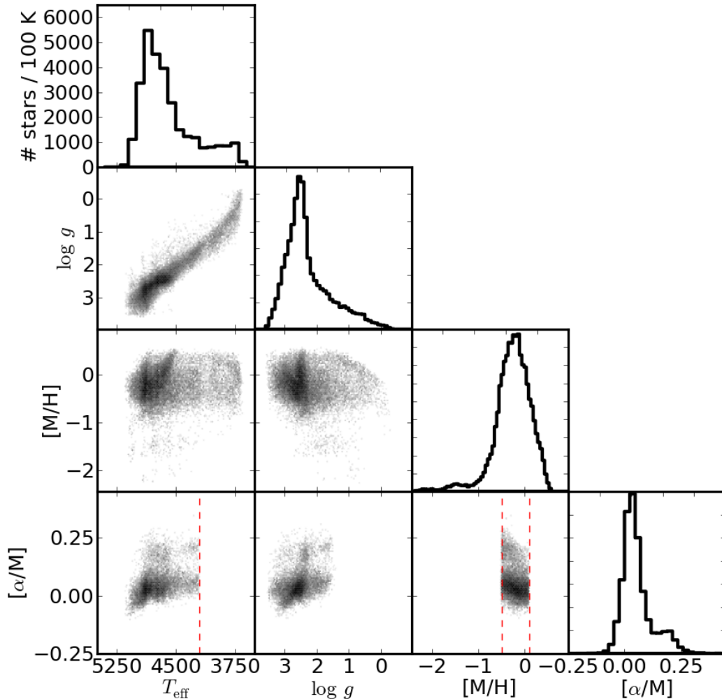
Figure 11. The one-dimensional and two-dimensional distributions of APOGEE stellar parameters — temperatures, surface gravities, metallicity, and [\alpha/M] — for all 29,438 APOGEE stars in DR10 which have reliable ASPCAP fits. The [\alpha/M] values are only shown for the 16,066 star subset with T_{\text{eff}} > 4200 K and -0.5 < [M/H] < +0.1 , which is the range for which [\alpha/M] values are reliable (limits are indicated by red dashed lines; see Section 3.7 for details). These distributions show what APOGEE has observed and ASPCAP has analyzed. They do not represent a fair sample of the underlying Galactic populations.
