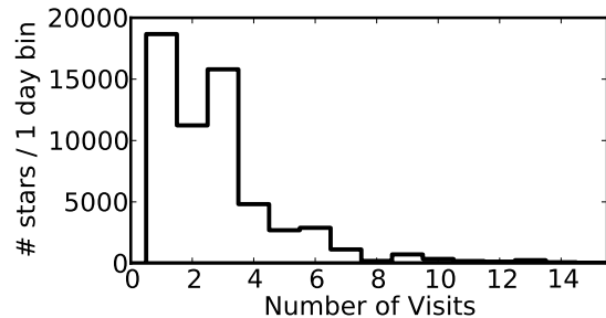
Figure 4. The distribution of number of spectroscopic visits for APOGEE stars included in DR10. While the bulk of stars have three or fewer visits, they may have reached our spectral S/N requirement if they are bright enough; see Figure 7.
