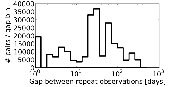
Figure 5. The distribution of time between visits for APOGEE stars, useful for determining the sensitivity to radial velocity variations due to binarity. This quantity is the absolute value of the time difference for all unique pairs of visits for each star. The most prominent peaks are at one and two months.
