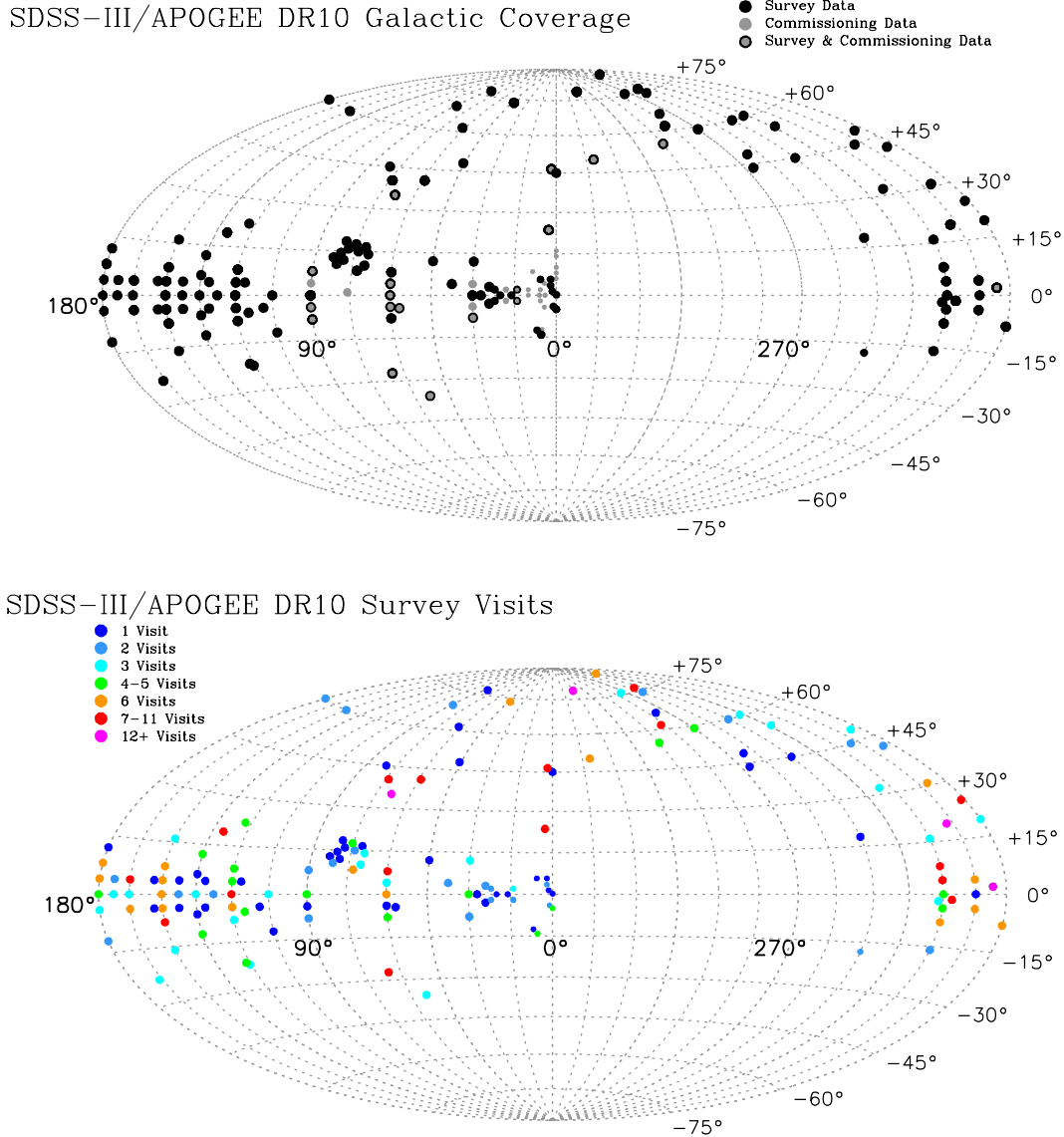
Figure 1. The distribution on the sky of all APOGEE DR10 pointings in Galactic coordinates: the Galactic Center is in the middle of the diagram. Each circle represents a pointing. APOGEE often has several distinct plates for a single location on the sky; DR10 includes 170 locations, which are shown above. Smaller circles (primarily near the Galactic Center) represent locations where plates were drilled over only a fraction of the 7 \text{ deg}^2 focal plane to minimize differential atmospheric refraction. Note the concentration of fields along the Galactic Plane. The concentration of pointings at l = 75^\circ, b = +15^\circ is a special program targeting stars observed by the Kepler telescope; see Section 3.4. (top) Distribution of pointings in both the commissioning and survey phases (both are included in DR10). (bottom) Pointings distinguished by the number of visits obtained by DR10 in the survey phase.
