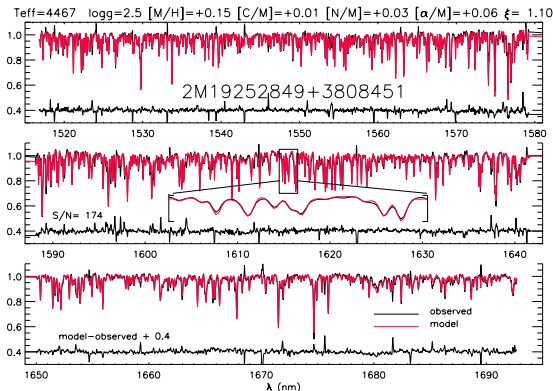
Figure 10. (upper lines) An example ASPCAP fit (red) to a typical APOGEE co-added stellar spectrum (black). (lower lines) Residual of the ASPCAP model fit compared to the data (offset from zero by +0.4 units for clarity of presentation). (inset) Zoom on a region showing the high resolution of the actual data. The H-band spectrum contains a wealth of information about the elemental abundances and stellar parameters of the star. The high resolution and high S/N of APOGEE spectra allow these atmospheric properties to be measured for the entire APOGEE sample.
