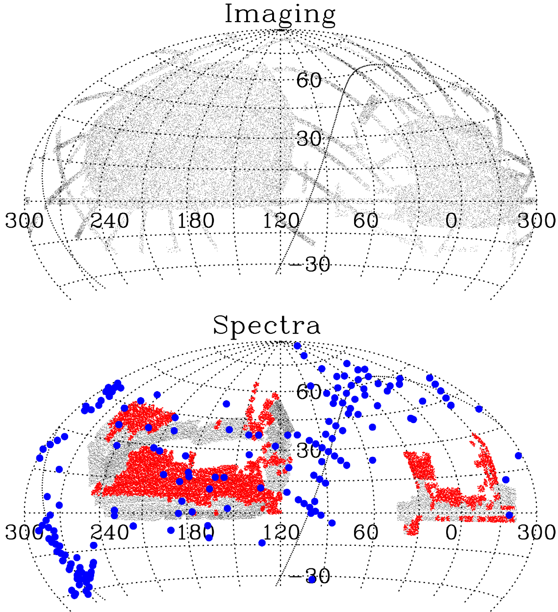
Figure 2. The distribution on the sky of all SDSS imaging (top; 14,555 \text{ deg}^2 – same as DR8 and DR9) and BOSS and APOGEE DR10 spectroscopy (bottom; 6373.2 \text{ deg}^2 ) in J2000 equatorial coordinates ( \alpha = 0^\circ is right of center in this projection). Grey shows regions included in DR9; the increment included in DR10 is in red. The blue shows the positions of APOGEE pointings included in DR10. The Galactic Plane is shown by the dotted line. The Northern Galactic Cap is on the left of the figure, and the Southern Galactic Cap on the right. The BOSS sky coverage shown is actually constructed using a random subsample of the BOSS DR10Q quasar catalog (Pâris et al. 2013). The sky below \delta < -30^\circ is never at an airmass of of less than 2.0 from APO (latitude= +32^\circ 46' 49'' ).
