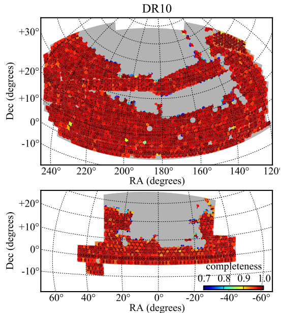
Figure 13. BOSS DR10 spectroscopic sky coverage in the Northern Galactic Cap (top) and Southern Galactic Cap (bottom). The grey region is the coverage goal for the final survey, totaling 10,000 \text{ deg}^2 . The color coding indicates the fraction of CMASS galaxy targets that receive a fiber; the fact that no two fibers can be placed closer than 62'' on a given plate reduces the average completeness to 94%. Note the higher completeness on the Equator in the Southern Galactic Cap (Stripe 82) where the plates are tiled with more overlapping area to recover collided galaxies.
