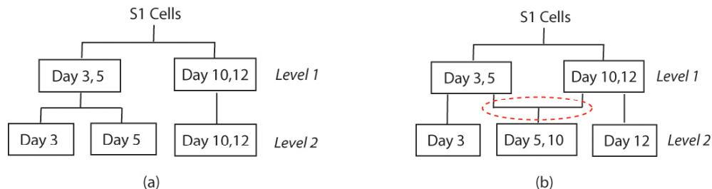
Figure 5. Illustration of the inconsistent phenotype grouping between successive levels. (a) Phenotype groupings at level 1 and level 2 are consistent. (b) Phenotype groupings at level 1 and 2 are inconsistent as the node Day 5,10 at level 2 is formed by breaking each of the node Day 3,5 and node Day 10, 12 into two parts and combining one part of node Day 3,5 with one part of Day 10,12. As long as the breaking operation is involved, the consistency between groups at successive levels is violated and the hierarchical structure cannot be represented as a tree.
