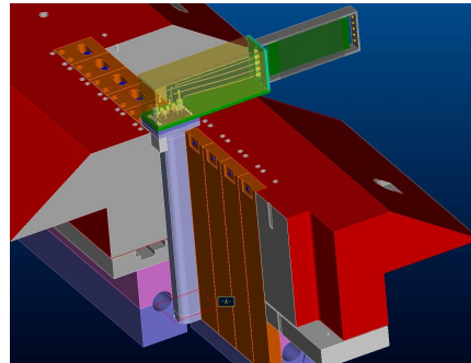
Fig. 2 – TAN installation
