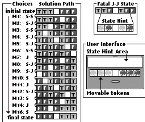
Figure 1: The Toads and Frogs problem
