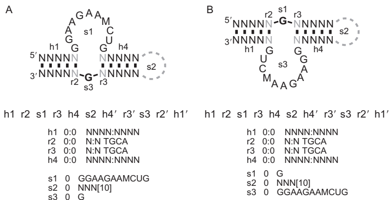
Figure 2.1 Secondary structure descriptors for an adenosine aptamer. The aptamer has been found to exist in both the 5' (A) and 3' (B) strands (Burgstaller & Famulok, 1994; Sassanfar & Szostak, 1993; Vu et al., 2012). The bulged guanosine nucleotide necessary for ligand binding is in bold.
