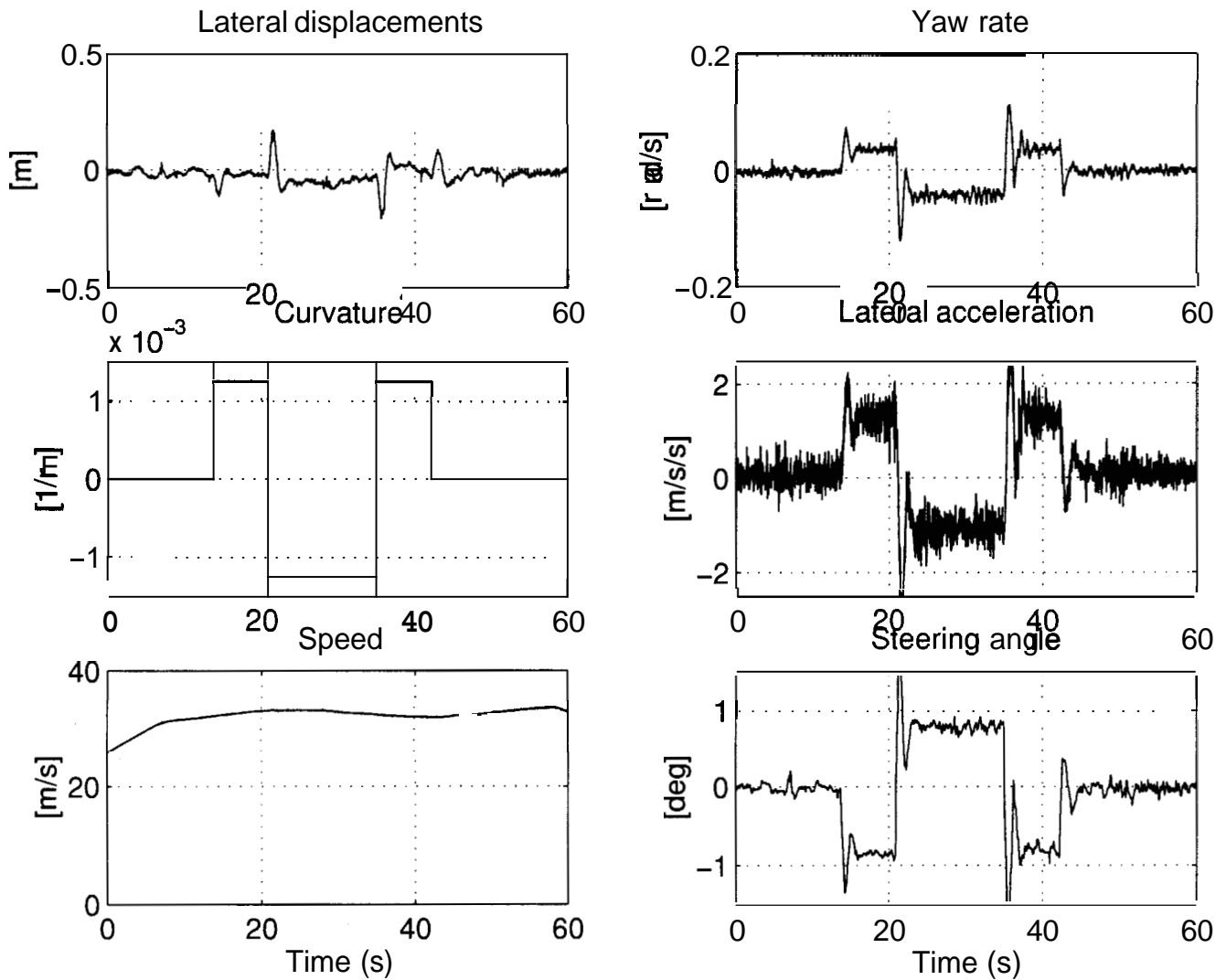
Figure 8: Controller performance with halved gains to simulate a wet road, with an integrator and with feedforward of road curvature
