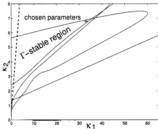
Figure 4: \Gamma -stability boundaries in the (\kappa_a, \kappa_b) -plane for the two representatives
