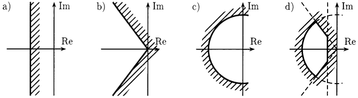
Figure 3: Basic elements of I?-stability: (a) settling time, (b) damping, (c) bandwidth. The combination of these basic elements (d) allows to fulfill several basic conditions simultaneously.
