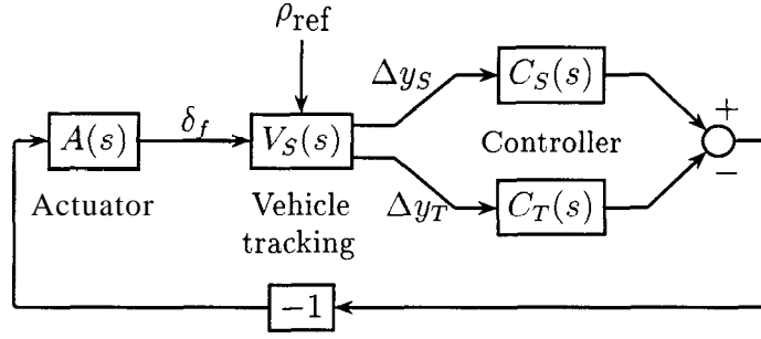
Figure 1: Block diagram of controller using front and tail lateral displacement measurements
