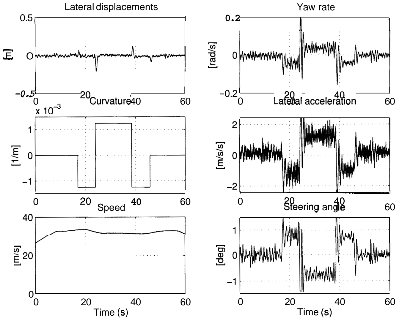
Figure 6: Controller performance on dry road, with an integrator and with feedforward of road curvature
