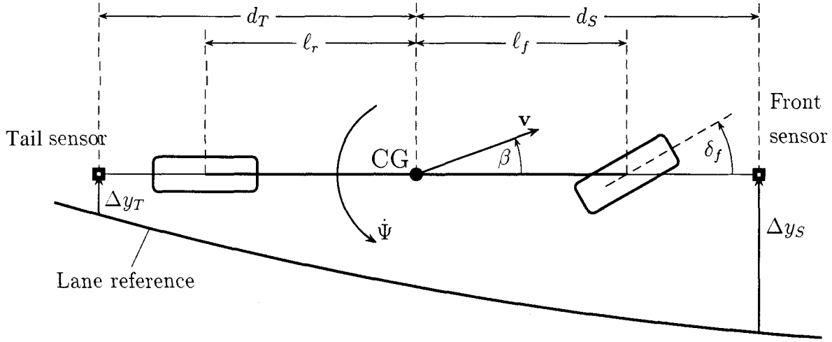
Figure 2: Single track model for automatic tracking
