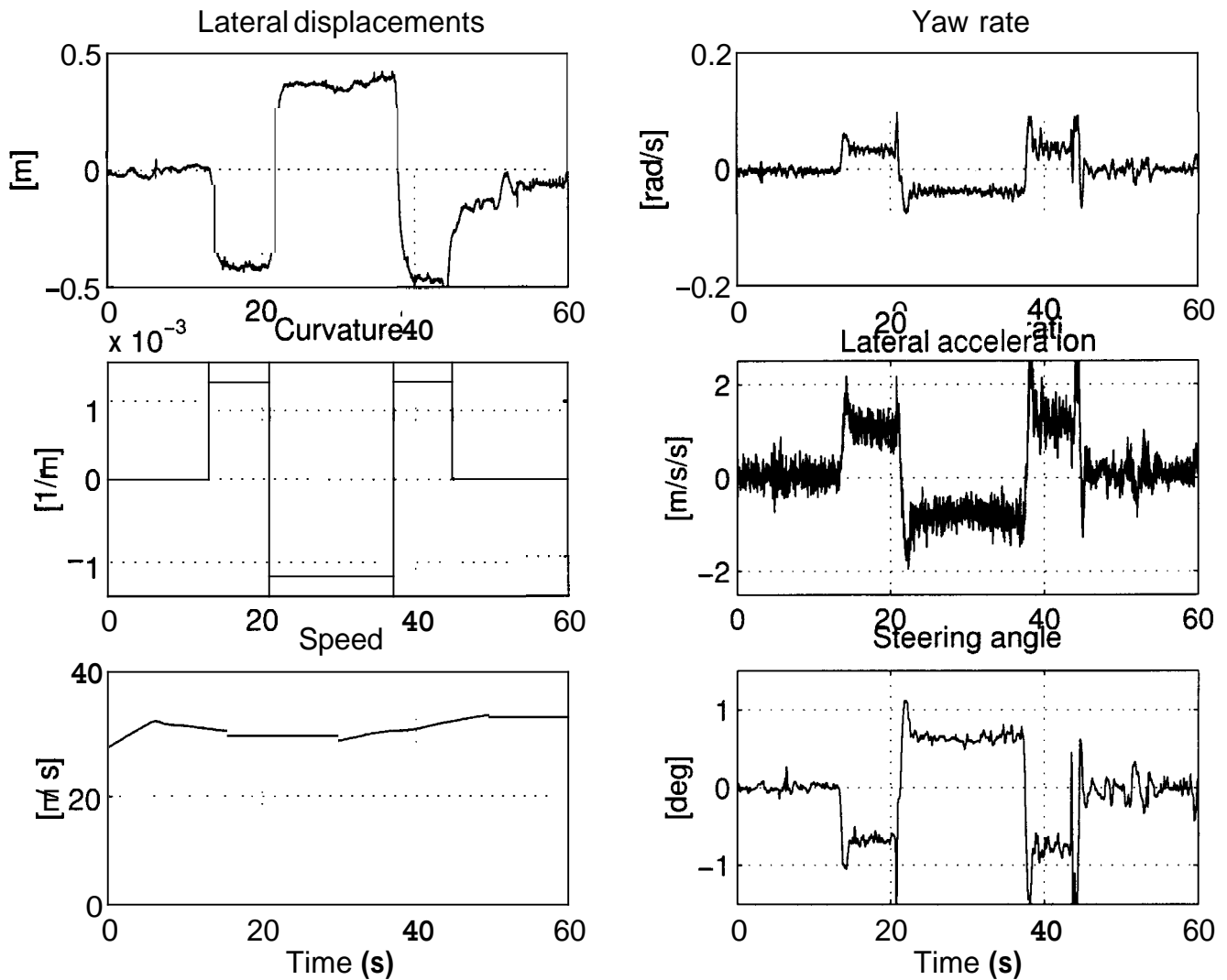
Figure 7: Controller performance with halved gains to simulate a wet road, without integral action and without road curvature preview
