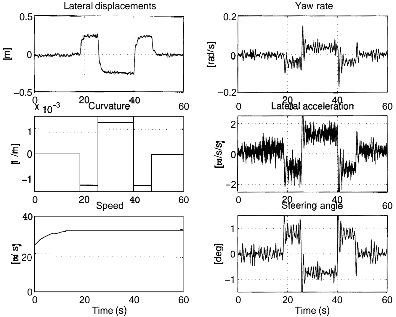
Figure 5: Controller performance on dry road, without integral action and without road curvature preview
