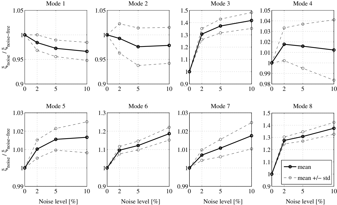
Fig. 14. Statistics (mean, mean +/- one standard deviation) over 100 trials of the identified damping ratios normalized to their counterparts identified based on noise-free data at different noise levels
