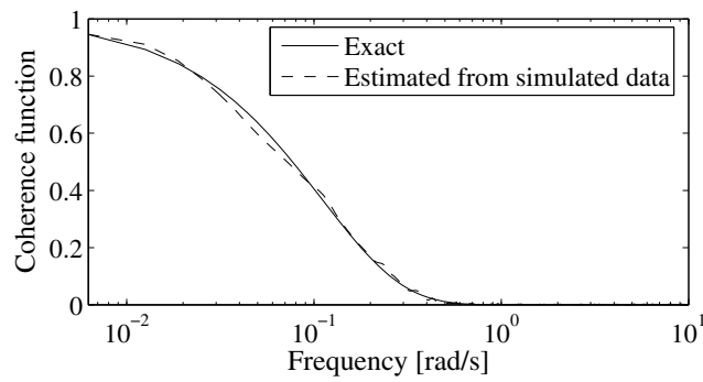
Fig. 7. Comparison of simulated and exact coherence function of the longitudinal wind velocity fluctuation
