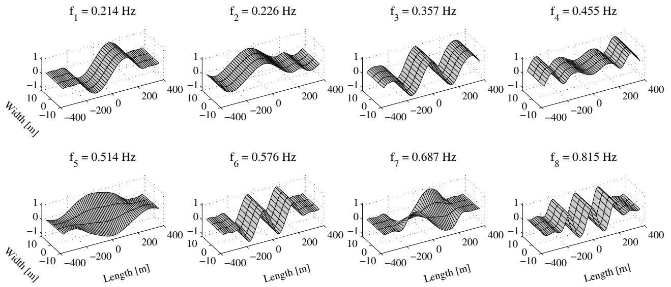
Fig. 11. 3D representation of normalized vibration mode shapes identified using SSI-DATA
