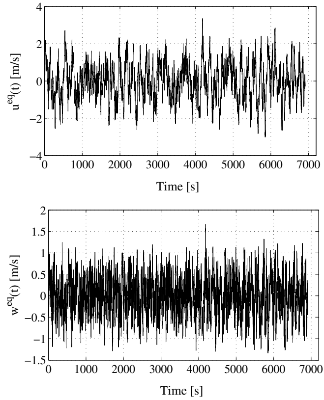
Fig. 5. Simulated longitudinal, u^{eq}(t) , and vertical, w^{eq}(t) , wind velocity fluctuations ( U = 10 m/s)
