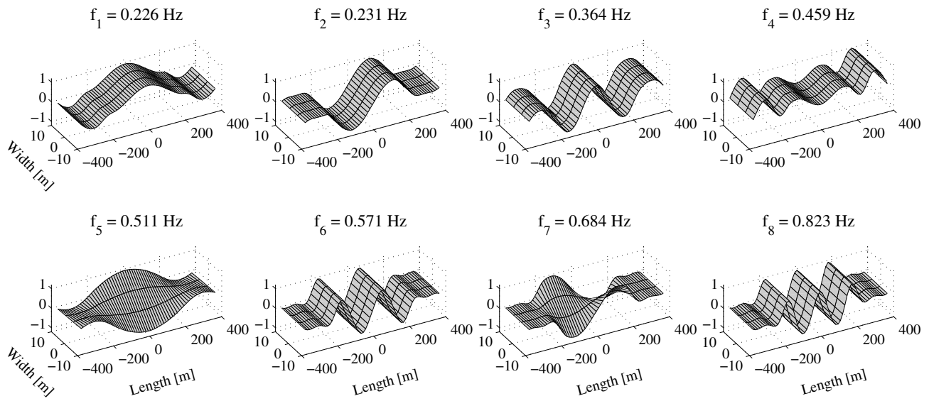
Fig. 12. 3D representation of vibration mode shapes computed from the finite element model of VTB
