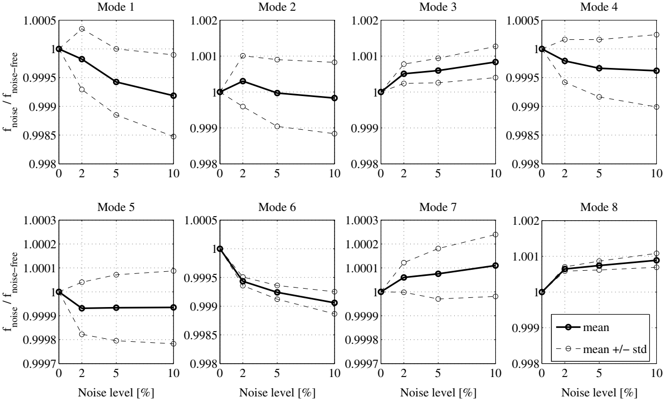
Fig. 13. Statistics (mean, mean +/- one standard deviation) over 100 trials of the identified natural frequencies normalized to their counterparts identified based on noise-free data at different measurement noise levels
