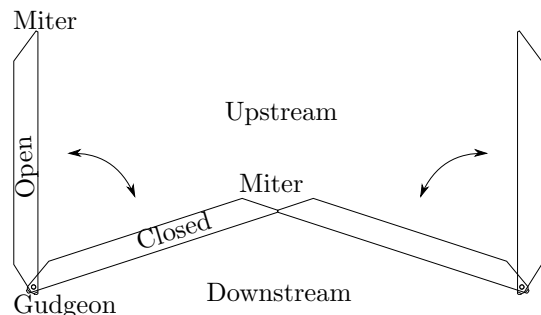
Fig. 8: Miter gate top view with swinging motion
