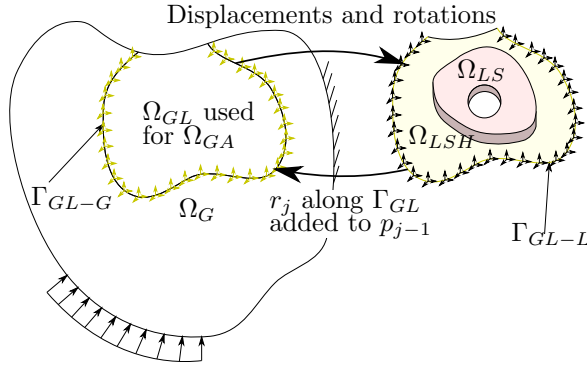
Fig. 6: Iterative global-local algorithm illustrated using \Omega_G , \Omega_{LSH} , \Omega_{LS} , feature of interest, \Gamma_N , Dirichlet boundary condition \Gamma_D , \Gamma_{GL-G} , \Gamma_{GL-L} , and \Gamma_{SH} . The top large arrow denotes application of displacements and rotations from the global solution to the local problem. The bottom large arrow denotes the application of the residual between a) the local solution reaction forces and moments and b) the global traction forces and moments to the global problem. This process is repeated until convergence is reached.
