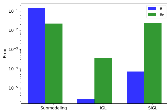
Fig. 28: SIF error e_K accuracy of submodeling, IGL and SIGL methods for a = 1 in, h_{up} = 50 ft, h_{down} = 16 ft, and l_{dmg} = 0.5 in.
