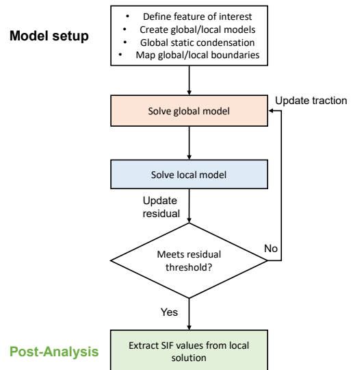
Fig. 2: Iterative global local overview.
