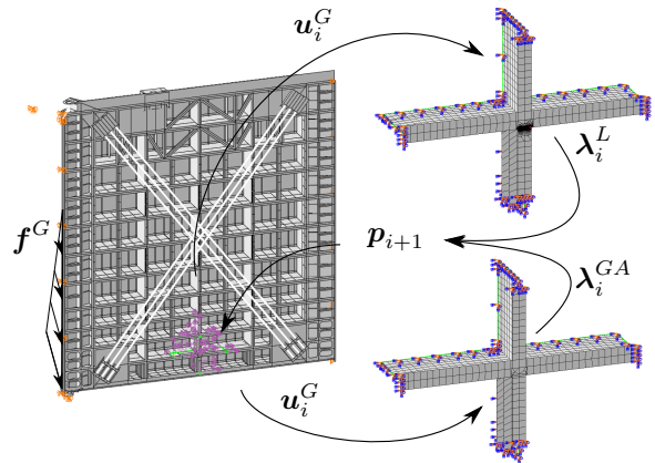
Fig. 17: Illustrated IGL fixed point iteration algorithm with Aitken's Delta-Squared method for miter gate with global, local, and global auxiliary mesh discretizations. The global domain has l_{dmg} , h_{up} , and h_{down} parameters. The local domain has parameter a .
