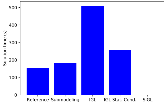
Fig. 29: Solution time for reference tying model, submodeling, IGL, IGL with global and auxiliary static condensation, and SIGL methods for a = 1 in, h_{up} = 50 ft, h_{down} = 16 ft, and l_{dmg} = 0.5 in.
