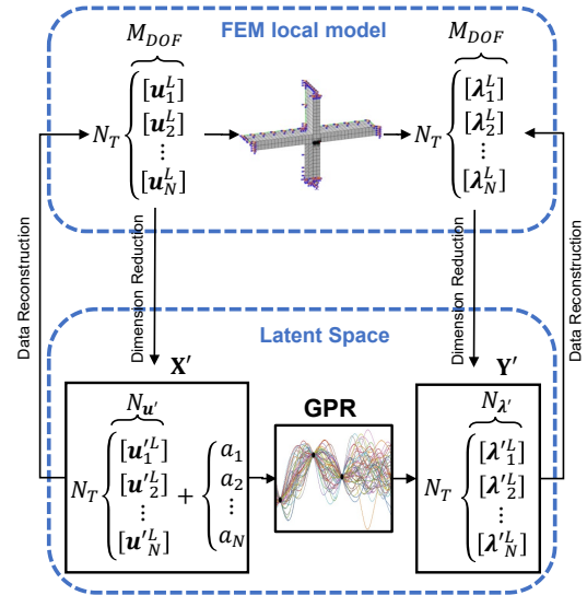
Fig. 19: Dimension reduction strategy of the proposed method compared with IO of FEM local model.
