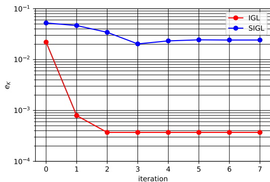
Fig. 27: SIF error e_K convergence of IGL and SIGL methods for a = 1 in, h_{up} = 50 ft, h_{down} = 16 ft, and l_{dmg} = 0.5 in.
