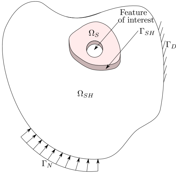
Fig. 4: Reference problem with shell domain \Omega_{SH} , solid domain \Omega_S , shell-to-solid tied boundary \Gamma_{SH} , feature of interest, Neumann boundary condition \Gamma_N , and Dirichlet boundary condition \Gamma_D
