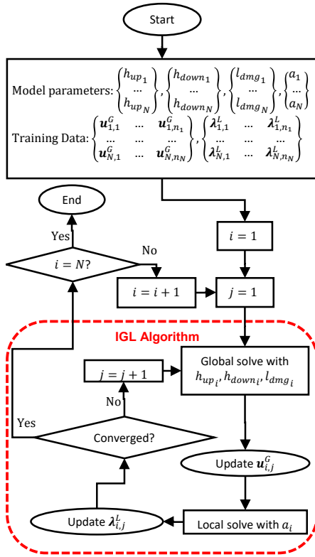
Fig. 18: Collecting \mathbf{u}^G , \boldsymbol{\lambda}^L , and SIF training data from the physics model.
