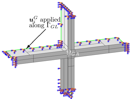
Fig. 16: Global auxiliary miter gate model. The global displacement solution u_j^G is applied along the global-local boundary \Gamma_{GL} .
