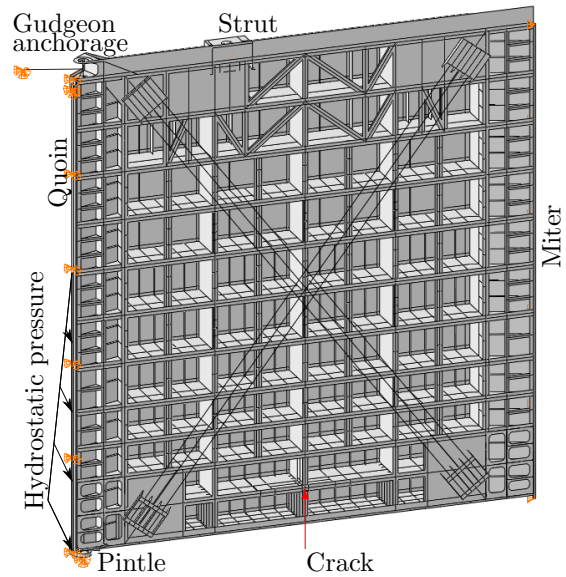
Fig. 10: Miter gate boundary conditions
