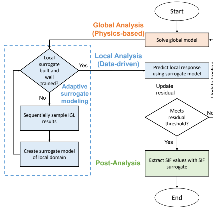
Fig. 3: Surrogate iterative global local overview
