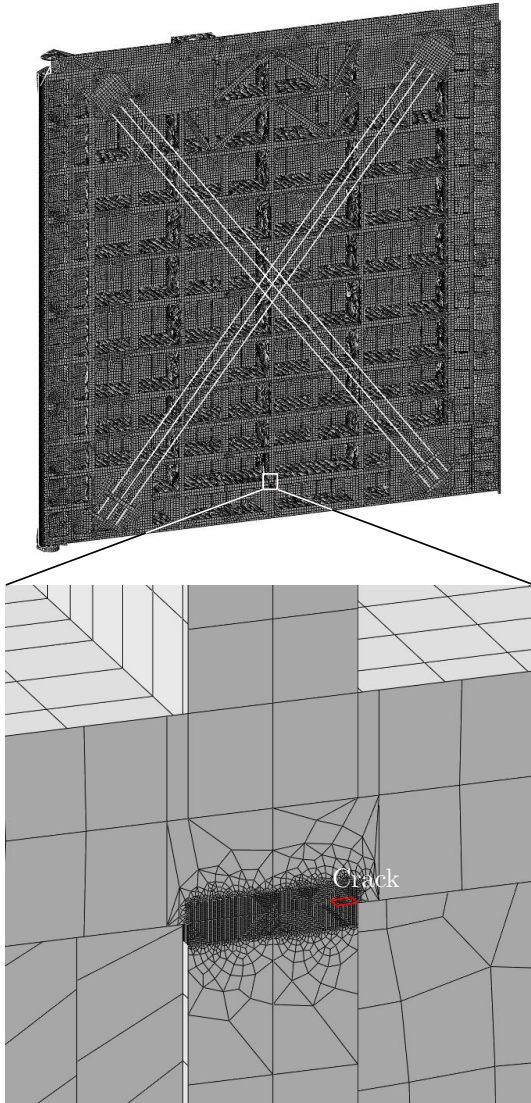
Fig. 13: Mesh discretization of reference miter gate model
