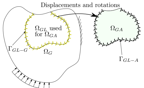
Fig. 7: Iterative global-local algorithm auxiliary domain \Omega_{GA} used for the calculation of global traction
