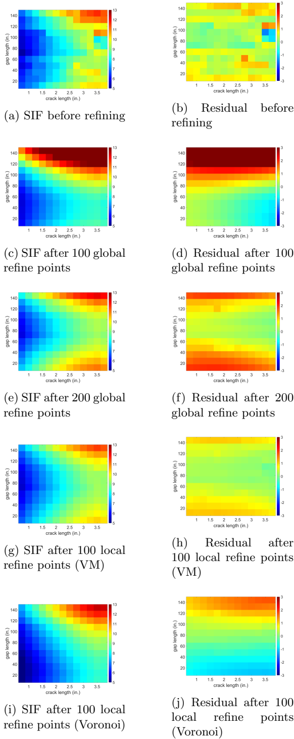
Fig. 31: SIF heatmaps showing S-IGL performance in \text{ksi}\sqrt{\text{in.}} .
