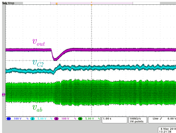
Figure 6.3: Experimental waveforms of PFC dc output voltage, v_{out} , v_{C2} , and buffer converter output voltage, v_{ab} during a slight load step (100 W to 150 W) implementing the band-pass filter based SSB control methods.
