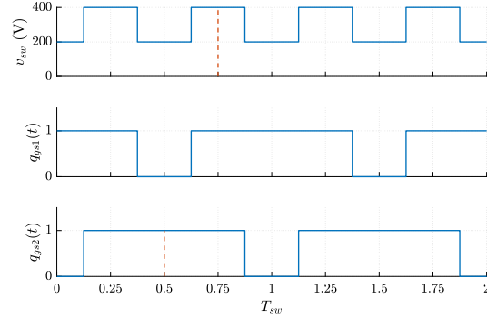
Figure 9.5: Three-level FCML switching waveforms with 0.75 duty ratio. The center of the switching node voltage is not aligned with the high level of PSPWM. Instead, the center of v_{sw} is phase shifted by \frac{1}{4}T_{sw} .
