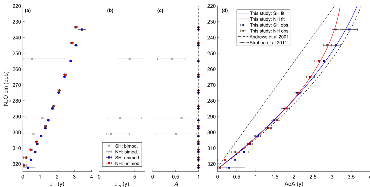
Figure 3. Hemisphere-specific properties of the age spectra in different N 2 O bins from the 10 s averaged airborne observations estimated by Markov chain Monte Carlo. Panels (a)–(c) show the value and 95 % confidence interval of \Gamma_1 , \Gamma_2 and A in each bin for either a unimodal (blue and red circles) or bimodal (faint blue and faint red stars) age spectrum depending on which type was preferentially selected by the algorithm. N 2 O values are offset by 1.4 ppb for all Northern Hemisphere estimates (NH, red) for visual clarity in panels (a)–(c). Panel (d) shows the mean AoA and confidence interval of the age spectra ensemble in each bin (i.e., unimodal and bimodal together). These data are fit by a quadratic polynomial for each hemisphere with a fixed y intercept (NH AoA = -0.0002381(323.23 - N_2O)^2 + 0.05567(323.23 - N_2O) ; SH AoA = -0.0001723(323.23 - N_2O)^2 + 0.05317(323.23 - N_2O) ). Previous relationships published by Andrews et al. (2001) and Strahan et al. (2011) are given as a dashed and dotted line for reference. y-intercept values of the previously published N 2 O–AoA calibrations have been updated to reflect the gradual increase in tropospheric N 2 O between 1997 and the new reference year 2009.
