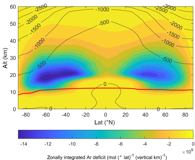
Figure 7. Color map of annual mean and zonally integrated Ar deficit in TOMCAT. Overlain black contour lines show \delta(\text{Ar}/\text{N}_2) (per meg). The red solid line highlights the mean position of the 200 hPa isobar.
