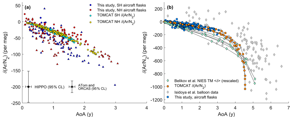
Figure 4. Comparison of age of air (AoA) and gravitational settling (GS) of \delta(\text{Ar}/\text{N}_2) in models and observations. Panel (a) shows observations from the Northern Hemisphere (red) and Southern Hemisphere (blue) together with TOMCAT model output (SH: cyan; NH: yellow) selected from the closest model grid box in time and space. Because uncertainty for AoA is similar for all stratospheric samples but \delta(\text{Ar}/\text{N}_2) uncertainty differs between campaigns, representative error bars (95 % confidence interval) are shown for HIPPO (triangles) and ATom/ORCAS (circles) at an arbitrary AoA. \delta(\text{Ar}/\text{N}_2) is normalized to yield a delta value of zero in the equatorial free troposphere. In panel (b), observations from airborne campaigns (this study) and the balloon sampling system (Ishidoya et al., 2008, 2013, 2018; Sugawara et al., 2018) are plotted with the AoA–GS relationship observed in TOMCAT and the NIES TM (Belikov et al., 2019) as lines for each of the latitude bands shown in Fig. 5 and points for different altitude bins between 10 and 35 km. To yield an equivalent estimate of \delta(\text{Ar}/\text{N}_2) , \delta(^{13}\text{CO}_2/^{12}\text{CO}_2) results from the NIES TM (Belikov et al., 2019) have been rescaled according to Eq. (5) and offset by \sim 10 per meg to account for the different tropospheric reference region in the definition of \delta .
