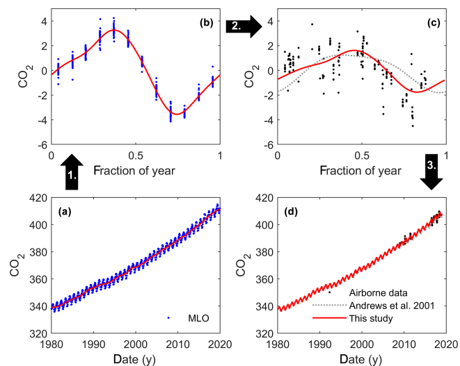
Figure 2. Illustration of the major steps in deriving a tropical upper tropospheric reference time series. Panel (a) shows the monthly mean surface CO 2 concentrations at Mauna Loa (MLO) (Keeling et al., 2001) with a stiff spline trend shown in red. Panel (b) shows a fit of the mean seasonal cycle at MLO compared to detrended observations from 1980 to 2019. Panel (c) shows the 1-month lagged seasonal cycle (red line) rescaled in amplitude to match detrended airborne observations in the equatorial upper troposphere (20° S < lat < 20° N, alt > 8 km, black). The seasonal cycle derived by Andrews et al. (2001) is presented as a dotted grey line for reference. Panel (d) shows the resulting upper tropospheric mean reference time series (TRTS, red) used for CO 2 in the age-of-air algorithm with the airborne observations from the tropical upper troposphere (black dots) and the time series (grey dotted line) of Andrews et al. (2001).
