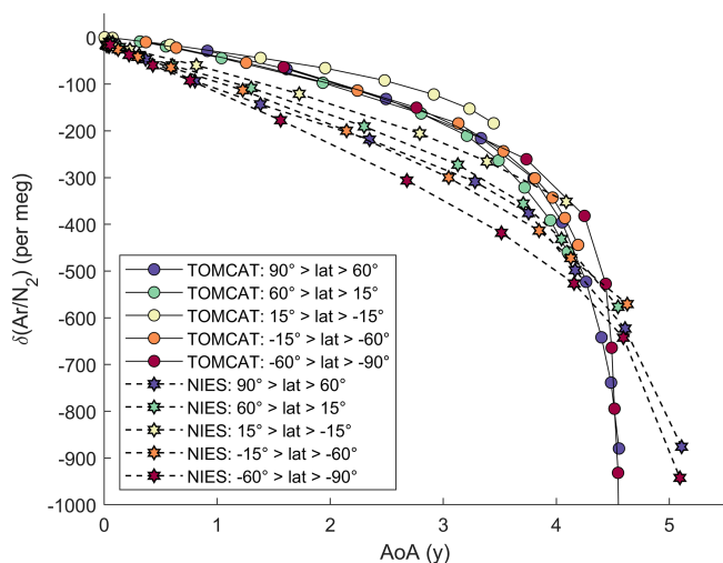
Figure 5. Comparison of the annual and zonal mean age of air (AoA) relationship with gravitational settling simulated in TOMCAT and the NIES TM. The relationship is plotted as lines for the latitude bands indicated by marker color. For the NIES TM, markers show the vertical profile using all grid boxes available between \sim 10 and 35 km. For TOMCAT, markers instead correspond to binned altitude bands between 10 and 35 km with a spacing of 2.5 km because of the finer vertical resolution of the model. To yield an equivalent estimate of \delta(\text{Ar}/\text{N}_2) , \delta(^{13}\text{CO}_2/^{12}\text{CO}_2) results from the NIES TM (Belikov et al., 2019) have been rescaled according to Eq. (5) and offset by \sim 10 per meg to account for the different tropospheric reference region in the definition of \delta .
