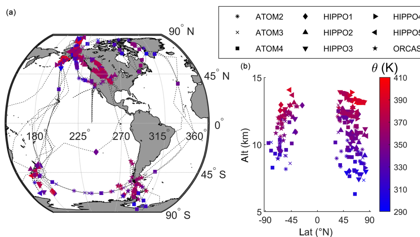
Figure 1. Horizontal (a) and vertical (b) distributions of airborne flask sample locations identified as being of stratospheric origin (see text). Thin dashed black lines on the map illustrate the flight tracks of all nine campaigns. Symbols indicate the campaigns during which the stratospheric samples were collected, and colors show the potential temperature at which the sample was taken.
