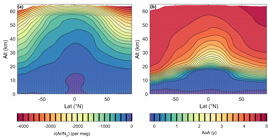
Figure 6. Annual and zonal means of \delta(\text{Ar}/\text{N}_2) (a) and age of air (AoA) (b) simulated by TOMCAT. Values of the contour lines are shown as black vertical lines on the color bar. Grey dots indicate the center of a grid box in TOMCAT. A video of this figure highlighting the natural variability in monthly-mean values is available in the Supplement.
