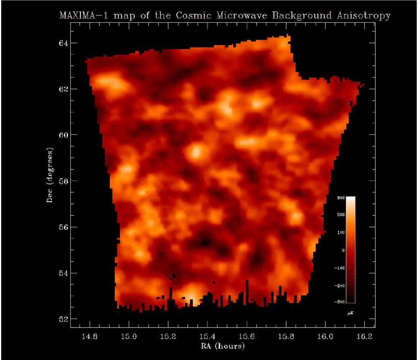
FIG. 1.— A Wiener filtered map of the CMB anisotropy with 10' resolution from MAXIMA-1. The map is made using data from three 150 GHz and one 240 GHz photometer and contains 15,000\ 5' \times 5' pixels. We used the angular power spectrum shown in the top panel of Figure 2 as the prior for the Wiener filter. Pixel boundaries have been smoothed using interpolation.
