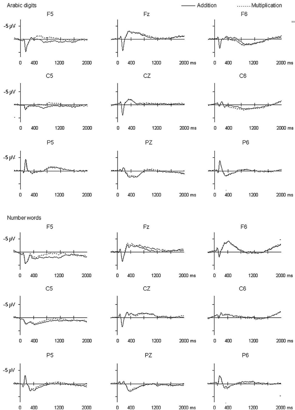
Fig. 5 – Event-related potentials for single-digit addition and multiplication at the left and right anterior, posterior scalp (experiment two). The top panel is for the Arabic digits condition, and the bottom panel is for the Chinese number words condition.
