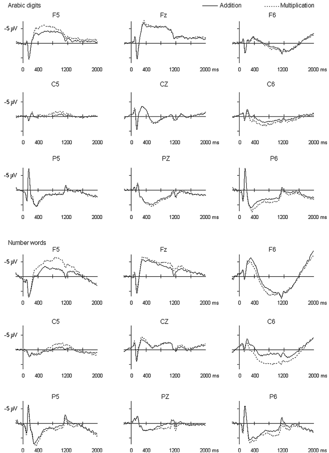
Fig. 2 – Event-related potentials for single-digit addition and multiplication at the left and right anterior, posterior scalp (experiment one). The top panel is for the Arabic digits condition, and the bottom panel is for the Chinese number words condition.
