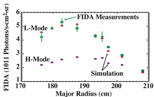
FIG. 2. Comparison of simulated profiles [H-mode (violet), L-mode (red)] and measured relative FIDA profile [L-mode (green)]. The FIDA signal is averaged over E_{\lambda} (energy component along the viewing line) between 20 keV and 40 keV.
