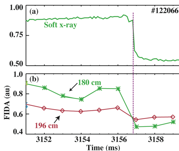
FIG. 4. Time evolution of (a) soft x-ray signal and (b) FIDA signals from two chords averaged over E_{\lambda} between 30 keV and 80 keV.
