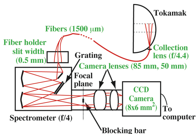
FIG. 1. Top view of the dedicated FIDA system.
