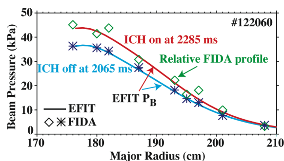
FIG. 3. Comparison of beam-ion pressure profiles and relative FIDA profile. The FIDA signal is averaged over E_{\lambda} between 40 keV and 80 keV.
