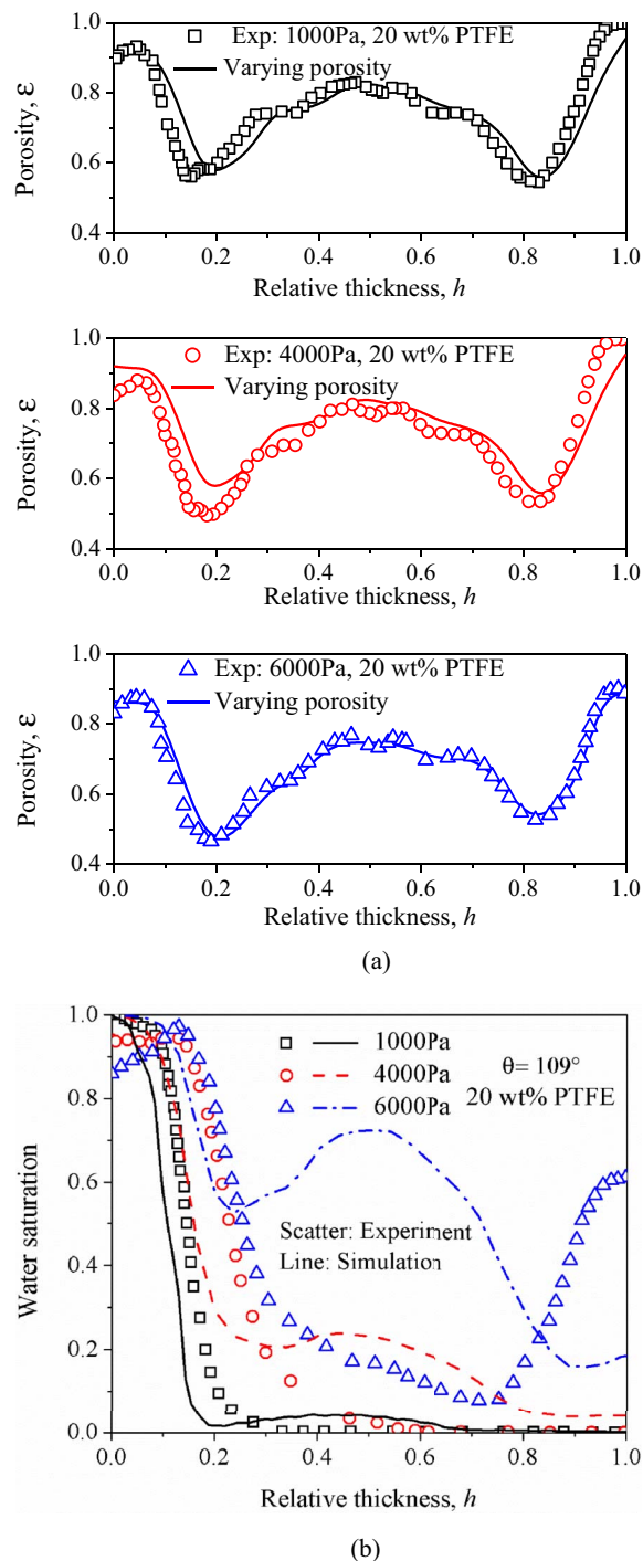
Figure 3. Comparisons of local porosity and water saturation over the through-plane direction between numerical results and X-ray experiment data. 8 Operating conditions: fiber contact angle \theta = 109^\circ , 20 wt% PTFE treatment for the GDL, \Delta p = 1000, 4000, 6000 \text{ Pa} . (a) Local porosity; (b) Local water saturation.
