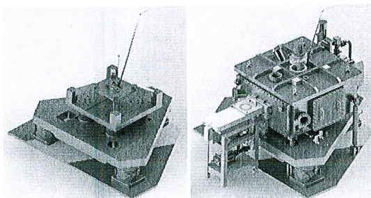
FIGURE 5. (Left) CAD model of SHARP's vibration-isolation system. (Right) Model of the assembled system. The beam path is shown in magenta. The green stripe represents the location of a buried grade beam.
