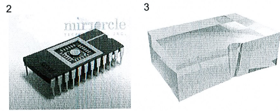
FIGURES 2 and 3. (2) Mirrorcle Technologies MEMS mirror, M_A . (3) Model of the elliptical M_C .
