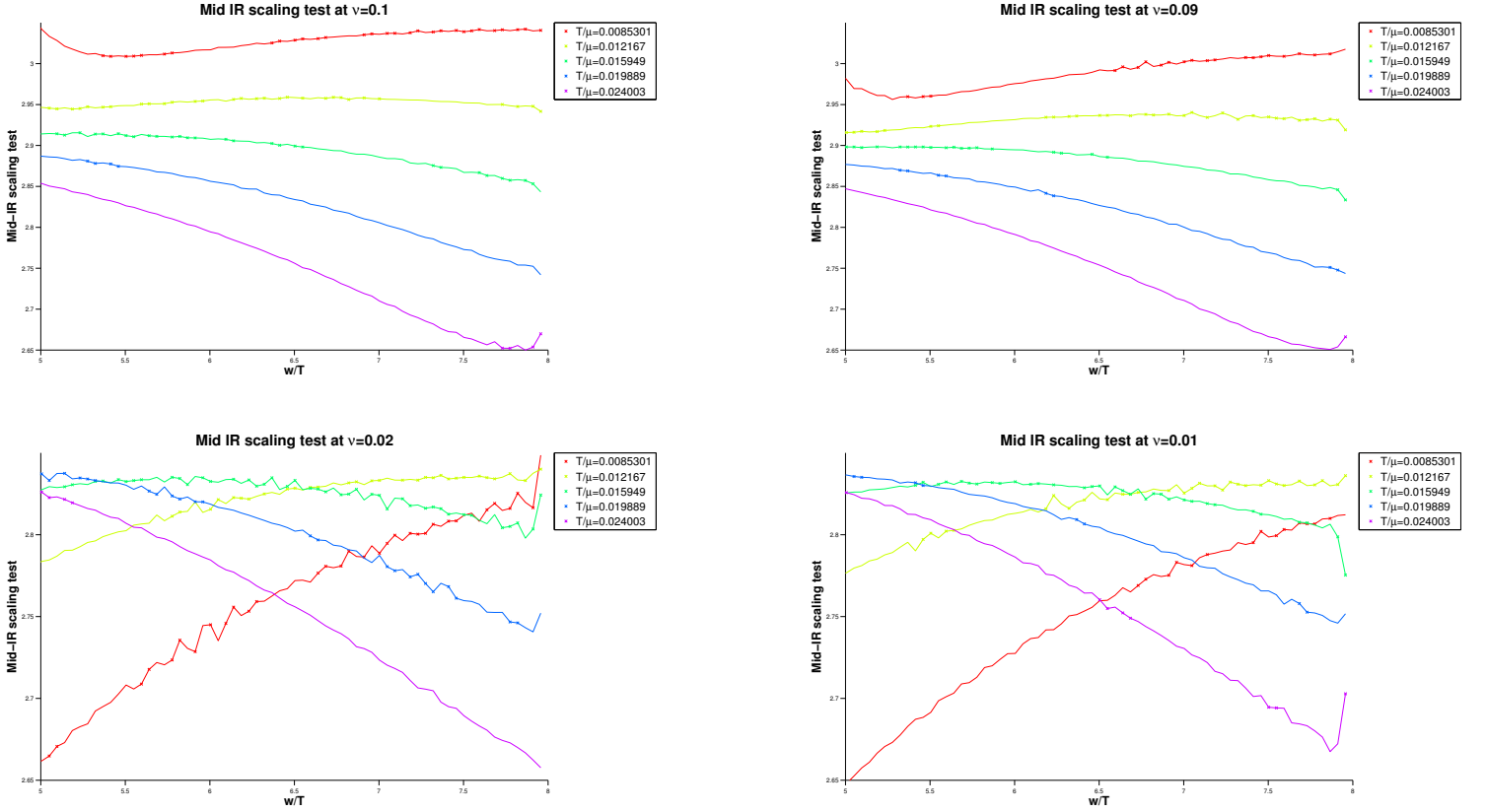
Fig. 10: The behaviour of the diagnostic function F(\omega) as we scan for mid-range scaling behaviour as a function of temperature. The reversal of the slopes of F(\omega) as a function of temperature, for a fixed v , imply that it should be possible to tune to a scaling regime by appropriately specifying the temperature.
