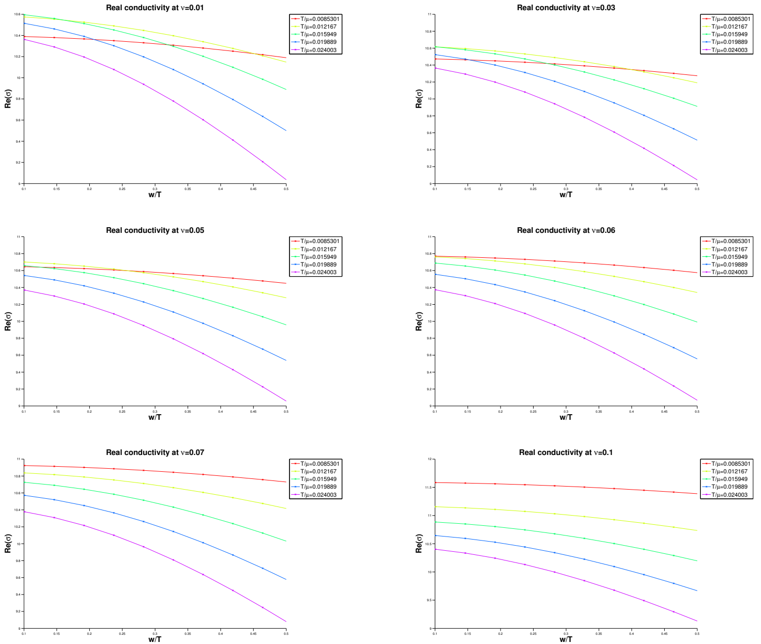
Fig. 8: Examining the real part of the AC conductivity as a function of \frac{T}{\mu} for a variety of \nu . At small \nu the constant \frac{T}{\mu} curves intercept and overlap for lower values of w . This can be interpreted as the AC representation of the incoherent phase. As \nu is increased the constant \frac{T}{\mu} curves separate and differentiate as we transition into a conducting phase.
