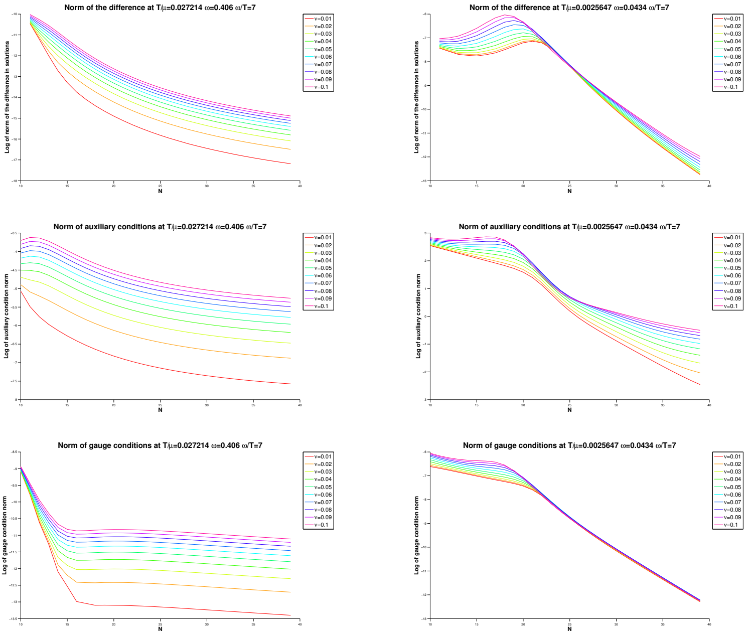
Fig. 19: Semi-logarithmic plots of the norm of the difference in solutions, and the norm of horizon auxiliary conditions and of the gauge conditions versus N at a low and high temperature for \frac{\omega}{T} = 7 . We note the unusual dual scaling regimes for the gauge conditions in the higher temperature case. More importantly we note the slow rate of convergence of the auxiliary conditions as the temperature is decreased.
