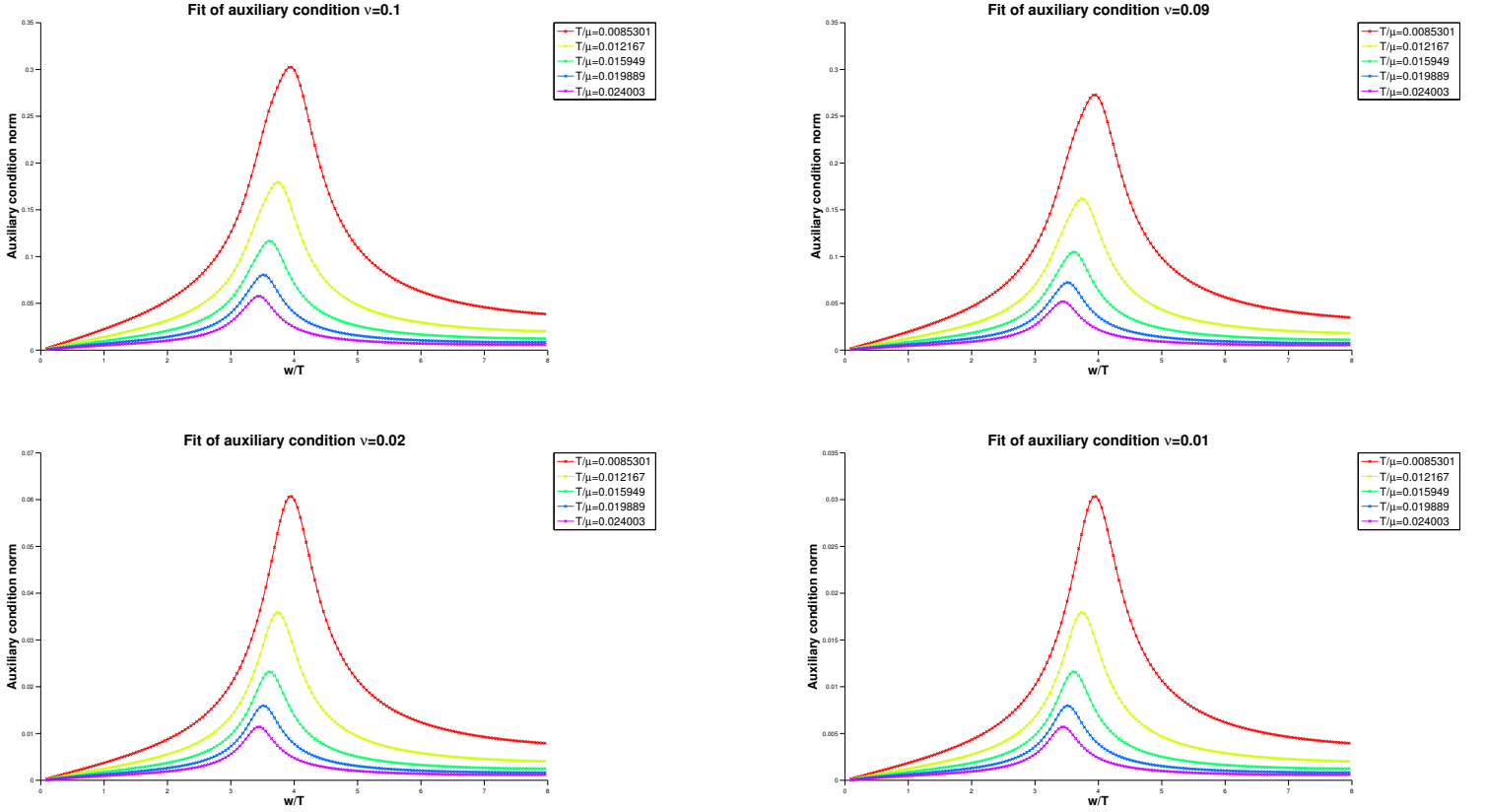
Fig. 23: The auxiliary horizon constraints corresponding to Fig 10. Again we observe the non-trivial dependence of the auxiliary constraints on the temperature, v and m with greater accuracy being obtained at lower and higher values of m .
