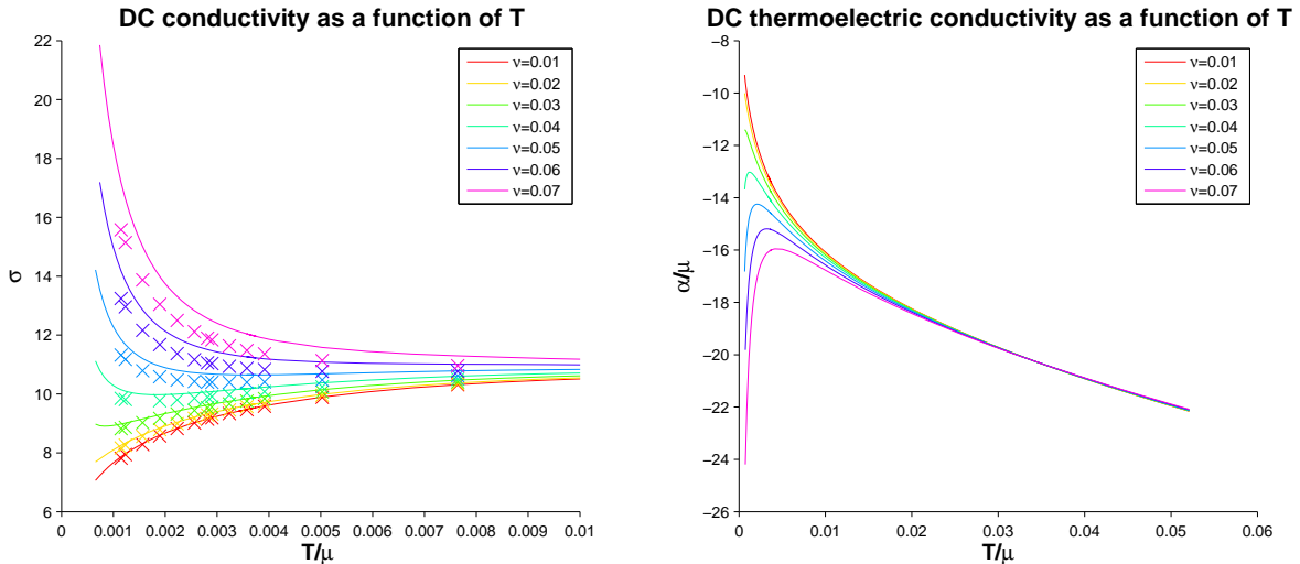
Fig. 1: Plots of the DC electrical and thermoelectric conductivities for a range of models against T for various theories parameterized by \nu , with C = 1.5, k = 1 held fixed. We clearly see the existence of the metallic and insulating regimes separated by an intermediate region.
