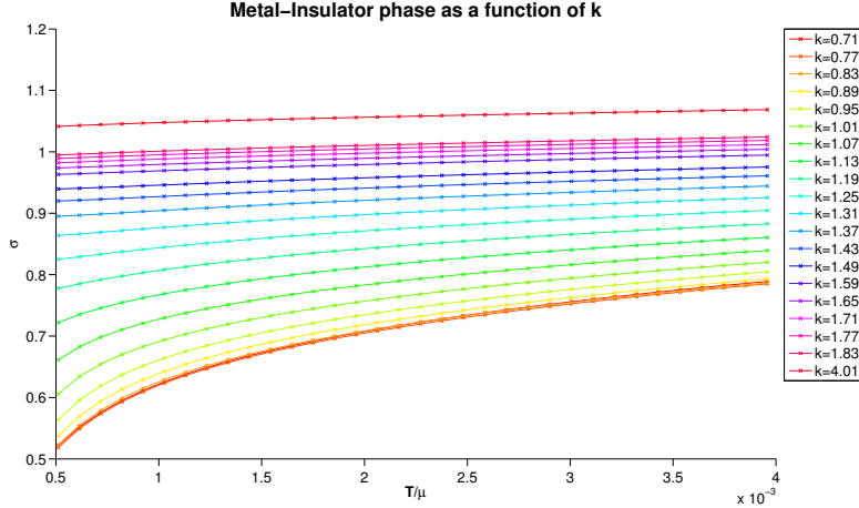
Fig. 6: The DC conductivity in the limit v = 0 for different lattices. We notice that for lower values of the wavelength k the conductivity is decreasing at low temperatures. As we increase k the DC conductivity begins to flatten at lower temperatures though for this choice of amplitude, C = 1.5 , for the sourced inhomogeneity the conductivity never transitions into the metallic phase for the temperatures which we can reliably access.
