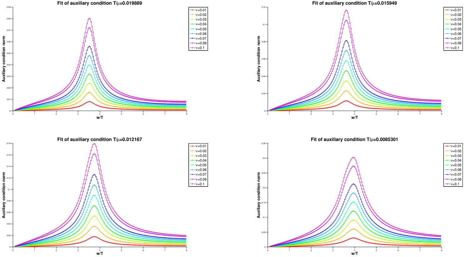
Fig. 22: The auxiliary horizon constraints corresponding to Fig 9. We see that while very well satisfied in the \mathfrak{w} \rightarrow 0 limit there is a regime of significant constraint violation prior to the return of greater accuracy in the mid IR.
