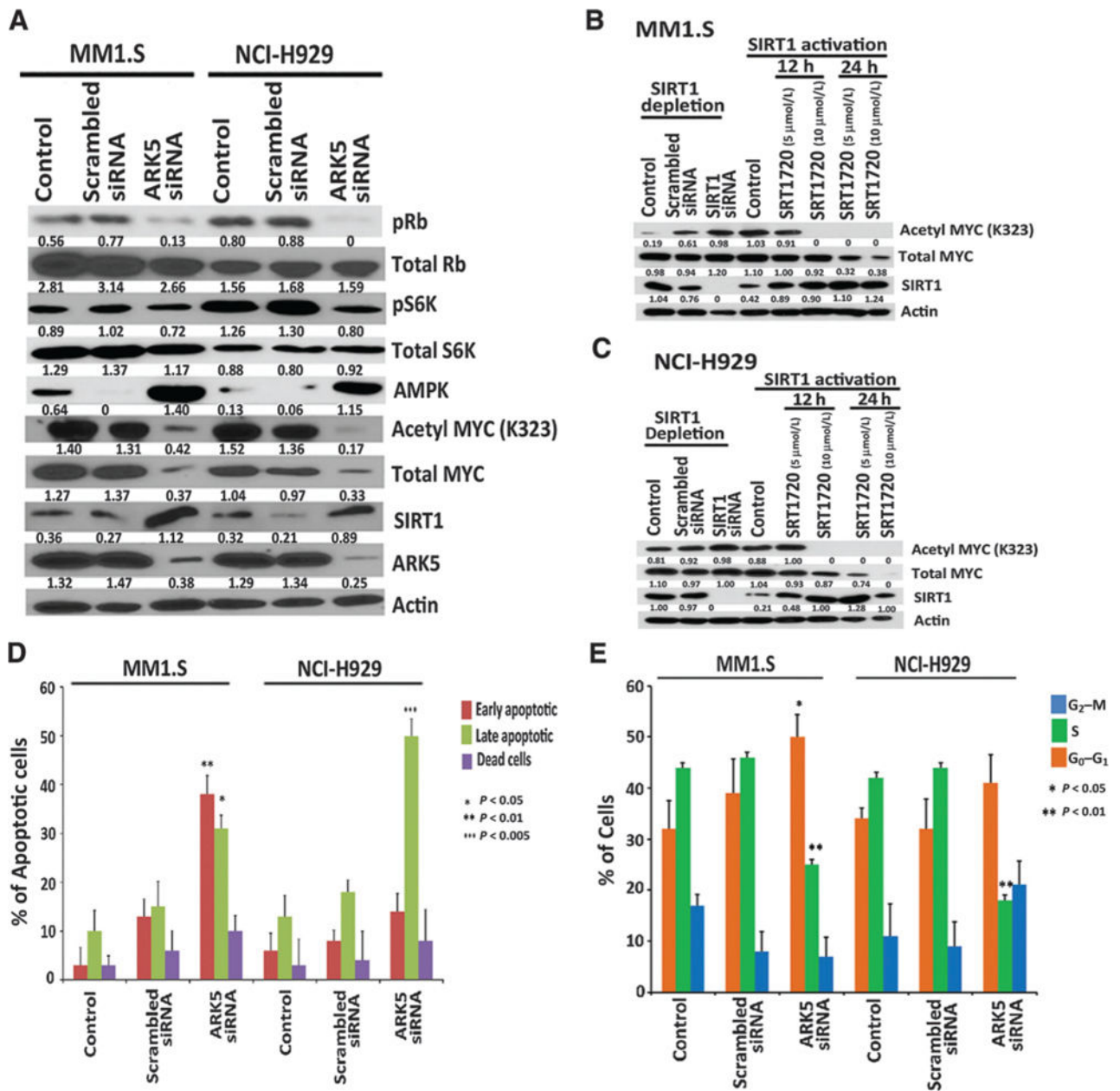
Figure 3. ARK5 depletion inhibits multiple myeloma cell growth via Rb/mTOR/MYC pathways and induces apoptosis and cell-cycle arrest. A, ARK5 repression significantly attenuated phosphoS6K, phosphoRb, MYC, and acetyl MYC activities in multiple myeloma. Conversely, depletion of ARK5 increased AMPK and SIRT1. Western blot analysis showing the levels of ARK5, SIRT1, MYC, acetyl MYC, total S6K, Rb, phosphoS6K, and phosphoRb proteins after 24-hour transfection in MM1.S and NCI-H929 siRNA-transfected cells. There was no difference in total Rb and total S6K between the groups. B and C, MM1.S and NCI-H929 cells were subjected to SIRT1 depletion by siRNA and SIRT1 activation with SRT1720. Western blotting confirmed that depletion of SIRT1 increased the acetylation activities of MYC, whereas the activation with SRT1720 resulted in decreased
