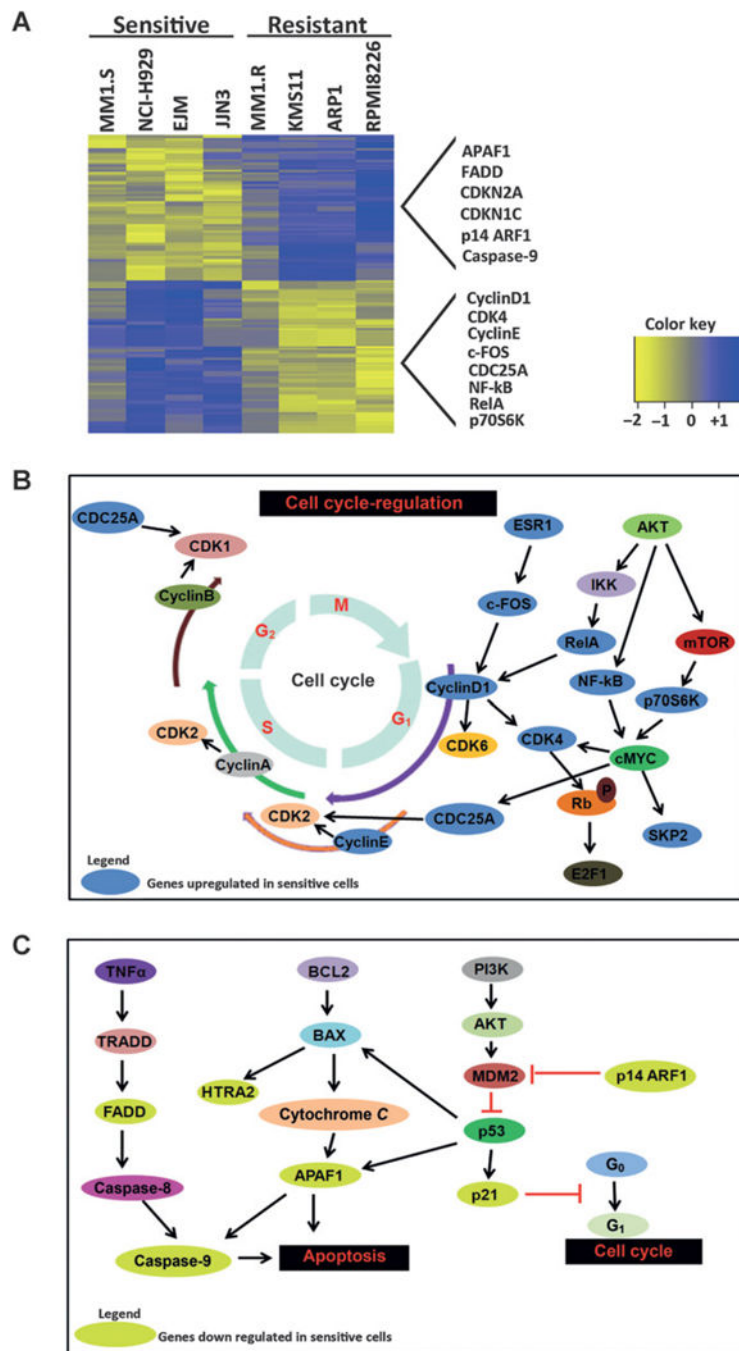
Figure 6. Transcriptomic profiling reveals cell cycle-regulated genes are highly enriched in ON123300-sensitive multiple myeloma cell lines. A, heatmap of 180 DEGs together with the indication about enrichment of MYC target genes in ON123300-sensitive multiple myeloma cell lines. B, molecular processes mediated by DEGs displaying altered expressions were sought using GeneGo program. Significant molecular biologic pathways were determined based on the analysis of significant biologic processes and expressions of the genes involved in these processes. As shown in the schematic, key cell-cycle regulators,
