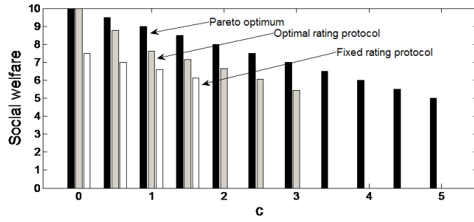
(b) L = 2
