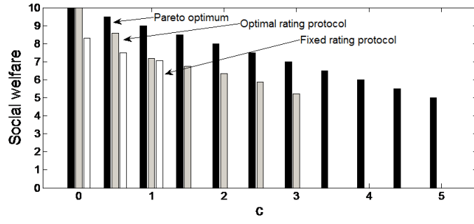
(a) L = 1
