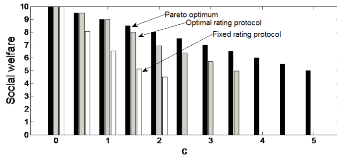
(c) L = 3
