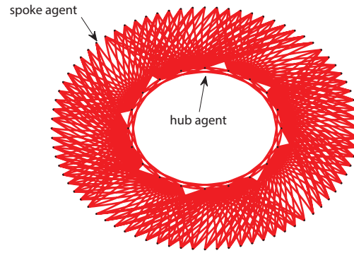
(a) k = 2
