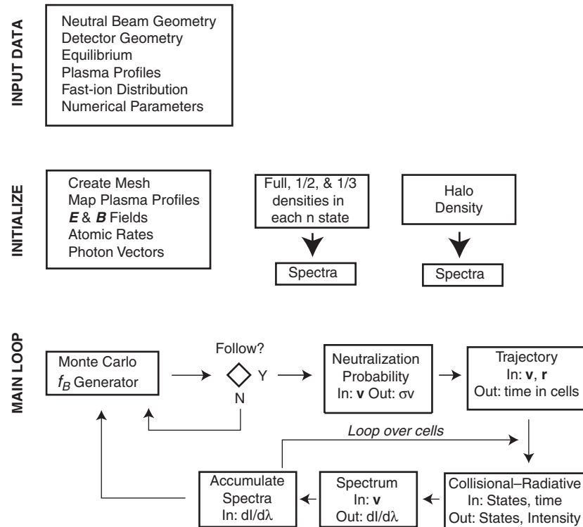
Figure 15. Flow diagram for the simulation code.
