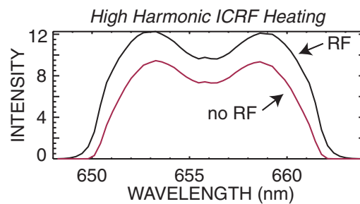
Figure 13. Approximate calculation of the spectral intensity, dI/d\lambda , for the fast-ion distribution that results from high-harmonic ICRF acceleration of the fast ions injected by a positive neutral beam for the geometry of figure 11. Typical DIII-D parameters for fourth harmonic ICRF acceleration of deuterium beam ions are assumed; the distortion of the beam slowing-down distribution is taken from the simple model of [44] for a case that doubles the neutron rate.
