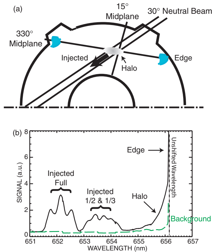
Figure 1. (a) Plan view of the DIII-D tokamak showing the modulated neutral beam source and the two sightlines for the data in this paper. Injected neutrals are in the beam ‘footprint’, warm halo neutrals are in a cloud around the injected beam, and cold edge neutrals are near the walls of the chamber. (b) Spectrum for the fibre that views the 30° modulated beam from the 330° midplane port when the beam is on (—) and off (- - -). The contributions to the spectrum of the injected, halo and edge neutrals are indicated.
