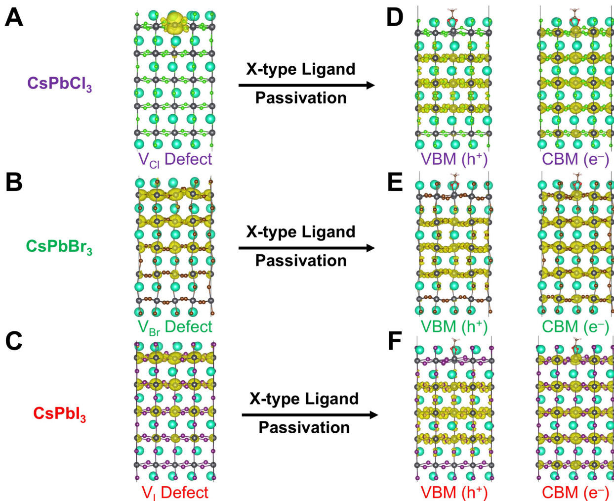
Figure 3. Charge density calculations at the HSE+SOC level of theory for (A) \text{CsPbCl}_3 with a surface chloride vacancy ( \text{CsPbCl}_3+V_{\text{Cl}} ), (B) \text{CsPbBr}_3 with a surface bromide vacancy ( \text{CsPbBr}_3+V_{\text{Br}} ), (C) \text{CsPbI}_3 with a surface iodide vacancy ( \text{CsPbI}_3+V_{\text{I}} ), (D) \text{CsPbCl}_3+V_{\text{Cl}} from (A) with a \text{CH}_3\text{COO}^- X-type passivating ligand, (E) \text{CsPbBr}_3+V_{\text{Br}} from (B) with a \text{CH}_3\text{COO}^- X-type passivating ligand, (F) \text{CsPbI}_3+V_{\text{I}} from (C) with a \text{CH}_3\text{COO}^- X-type passivating ligand. VBM and CBM states are unaffected by surface halide vacancies in (A), (B), and (C), and thus are excluded. In all cases, X-type passivation of halide-deficient surfaces yields a trap-free bandgap with fully delocalized VBM and CBM states. Cs, Pb, Cl, Br, I, O, C, and H atoms are shown as blue-green, gray, green, orange, purple, red, brown, and white, respectively.
