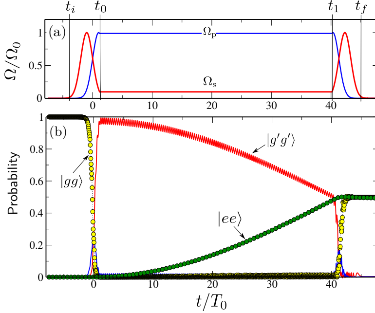
Figure 3. IR-dressed two-qubit gate in the rotating frame. (a) Raman pulse sequence with Stokes pulse \Omega_s(t) preceding the Pump pulse \Omega_p(t) . At time t_0 the mixing angle \alpha_0 with \sin \alpha_0 = 0.995 is established. The pulse intensities are then kept constant for a time interval \tau_e = \pi/4J . At time t_1 the pulse sequence is reversed to return the population to the original computational subspace \{|g\rangle, |e\rangle\}^{\otimes 2} . (b) Two-qubit state evolution in the subspace \{|g\rangle, |e\rangle, |f\rangle, |g'\rangle\}^{\otimes 2} , associated with the pulse profile in panel (a), for the input state |g_1g_2\rangle . The pulse sequence performs an almost complete population transfer |g\rangle \rightarrow |g'\rangle at time t_0 . The dipole-dipole interaction between molecules performs the gate U_{12}(t) = \exp[-iJX_1X_2t] , populating the state |e_1e_2\rangle . At time t_1 the inverse mapping |g'\rangle \rightarrow |g\rangle is performed, leading to the output state U_{12}(\tau_e)|g_1g_2\rangle . The gate fidelity is \mathcal{F}_{gg} \equiv |\langle \Phi_{gg} | U(\tau_e) | gg \rangle| , with the ideal output |\Phi_{gg}\rangle = (|g_1g_2\rangle - |e_1e_2\rangle)/\sqrt{2} . \mathcal{F}_{gg} \approx 0.99 in this example. t_g = t_f - t_i is the total gate time, J = 0.02 T_0^{-1} is the interaction energy and X_i is a Pauli operator. The qubit energy splitting \epsilon = \epsilon_e - \epsilon_g is zero during the gate operation.
