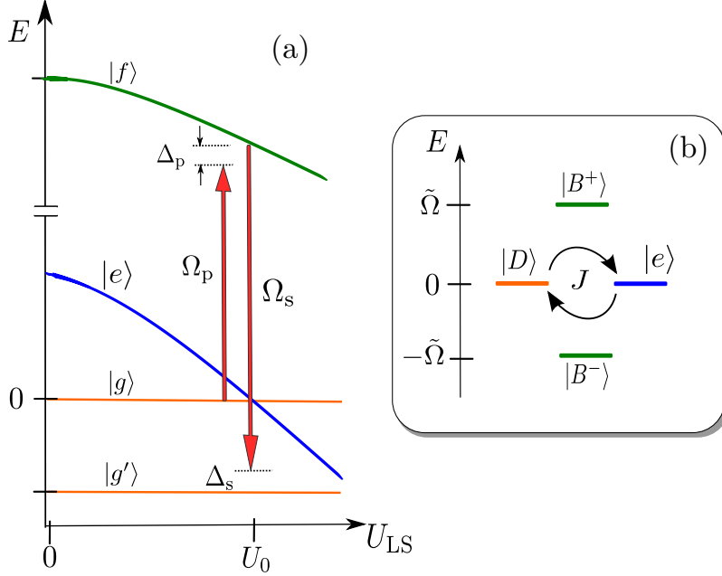
Figure 2. Level scheme used for infrared dressing. (a) Schematic level diagram for the subspace \{|g'\rangle, |g\rangle, |e\rangle, |f\rangle\} as a function of the tensor lightshift U_{LS} . For U_{LS} = 0 , the energies are given by the Zeeman spectrum in Fig. 1. The two ground states |g\rangle and |g'\rangle are coupled to the vibrationally excited state |f\rangle . The laser coupling is characterized by the Rabi frequencies \{\Omega_p, \Omega_s\} and detunings \{\Delta_p, \Delta_s\} . The state |e\rangle has a tunable gap \epsilon_e from state |g\rangle and is not coupled to |f\rangle by the dressing fields. States |e\rangle and |g\rangle become degenerate when U_{LS} = U_0 . (b) For U_{LS} = U_0 , the state |e\rangle is degenerate with the dark-state |D\rangle = \alpha_1|g\rangle + \alpha_2|g'\rangle , forming a two-level subspace in which dipole exchange processes occur at the rate J . Bright states |B^\pm\rangle involving the excited state |f\rangle are separated from the \{|D\rangle, |e\rangle\} subspace by a gap \tilde{\Omega} \gg J .
