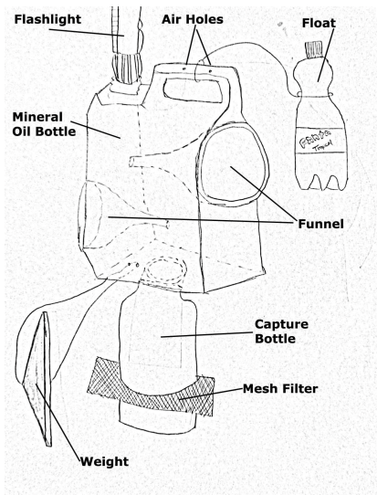
FIGURE 1. Schematic of the light trap used in this study.
