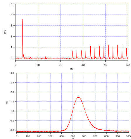
Figure 6. Postprocessed data. ALS train, camshaft bunch and parasitic bunch (top), detail of camshaft (bottom).
