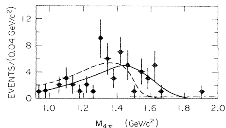
FIG. 2. 3\pi^\pm\pi^0 invariant-mass distribution for the selected decays. The curves are drawn for m_{\nu_\tau} = 0 (solid) and 250 MeV/ c^2 (dashed) and with the assumption that the four-pion state is dominated by a \rho' resonance of mass 1570 MeV/ c^2 and width 510 MeV/ c^2 . The dash-dotted line represents the hadronic background.
