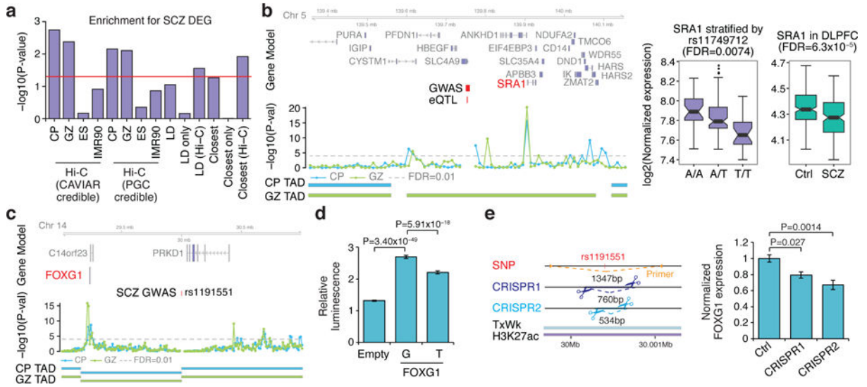
Figure 4. Functional validation of schizophrenia risk genes predicted by Hi-C a , Over-representation of schizophrenia risk genes with downregulated genes in schizophrenia DLPFC. Hi-C: CP, GZ, ES, IMR90, genes that are associated with CAVIAR credible SNPs or originally identified credible SNPs (PGC credible) in each tissue/cell type; LD, genes that are in LD with index SNPs, that are identified (LD, Hi-C) and not (LD only) by Hi-C; closest, closest genes to index SNPs, that are identified (closest, Hi-C) and not (closest only) by Hi-C. b , Hi-C interactions and eQTL association identify the same gene (left, marked in red), which is dysregulated in the same direction in schizophrenia DLPFC (right). Coordinates for the 10 kb bin containing credible SNPs (schizophrenia GWAS) and eQTL are indicated. Whiskers, 1.5 \times interquartile range; centre lines, median. c , Interaction map of SNP rs1191551 indicates an interaction with FOXG1 . d , rs1191551 risk allele (T) decreases luciferase activity (mean \pm standard error, n = 32 ). P values, linear mixed effect model. e , Predicted cleavage sites for two guide RNA pairs (CRISPR1 and CRISPR2); location of primers used to validate deletion are indicated. Rs1191551 is located in a weakly transcribed region (TxWk) containing a predicted active enhancer (H3K27ac) in fetal brain (left). CRISPR/Cas9-mediated deletion of rs1191551 flanking region reduces the expression of FOXG1 (right). Normalized expression levels of FOXG1 relative to control (Ctrl) (mean \pm standard error, n = 6 (Ctrl), 4 (CRISPR1 and CRISPR2)). P values, one-way ANOVA and post hoc Tukey test.
