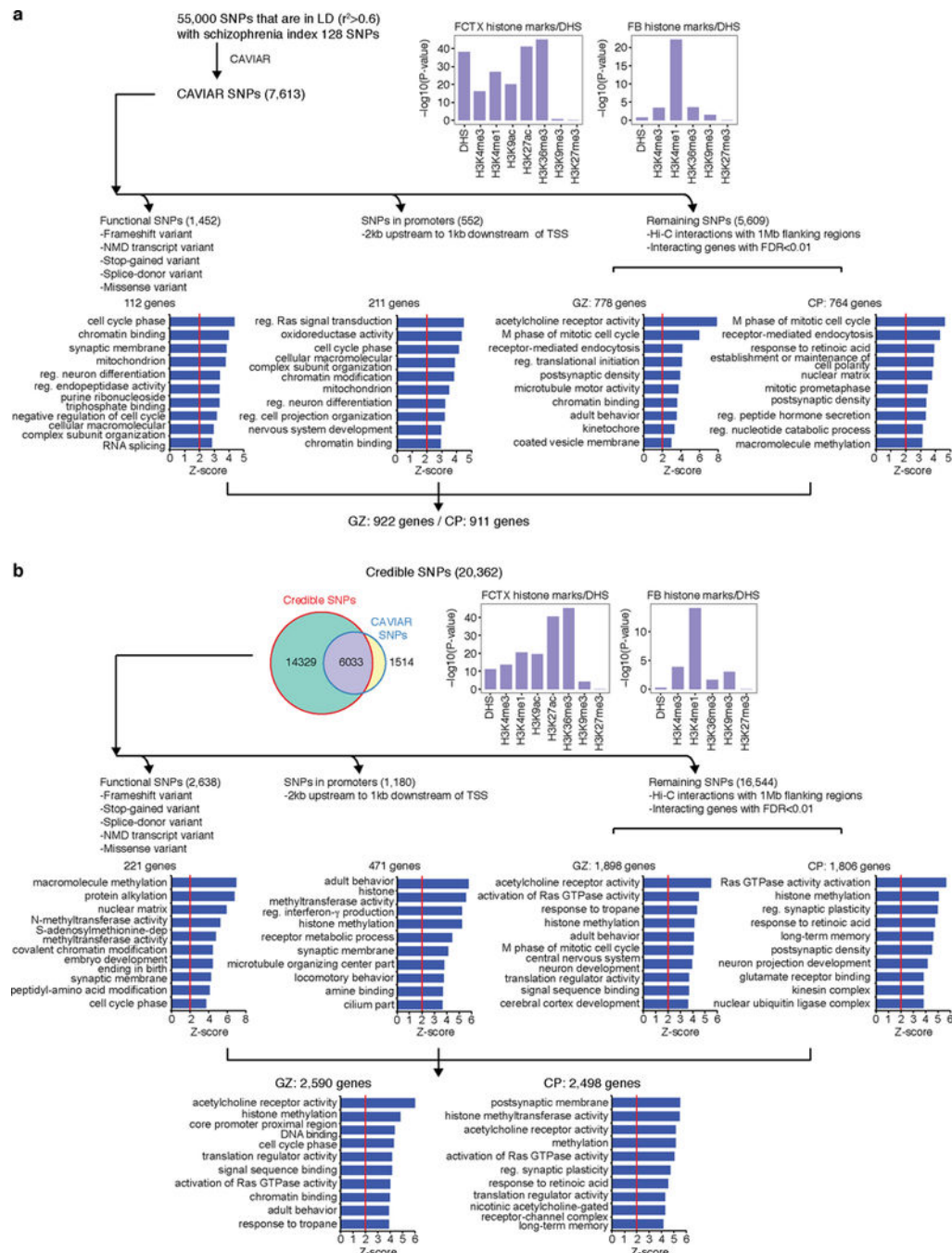
Extended Data Figure 7. Defining schizophrenia risk genes based on functional annotation of credible SNPs
