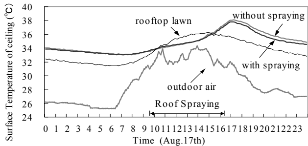
Figure 11 Ceiling surface temperatures
