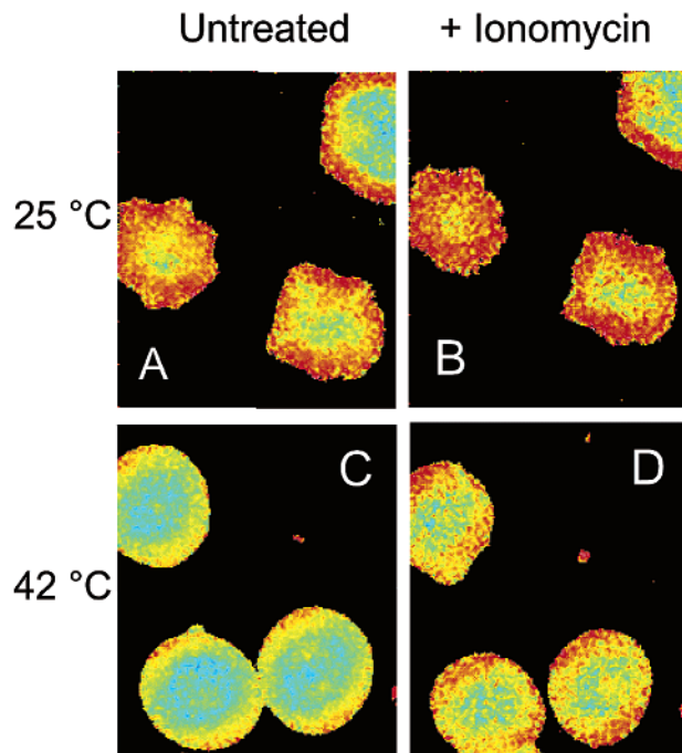
FIGURE 4: Two-photon excitation microscopy images of the effects of ionomycin and sPLA 2 on laurdan GP in erythrocyte membranes at 25 and 42 °C. Cells were treated and images acquired as described in Experimental Procedures. Parts A and C: untreated cells. Parts B and D: cells treated ~350 s with ionomycin. Blue represents the lowest values of GP (least ordered), and red represents the highest (most ordered).
