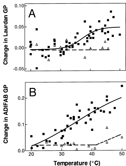
FIGURE 3: Temperature dependence of the change in laurdan fluorescence (A) or hydrolysis (B) in erythrocyte membranes change upon addition of ionomycin. Part A: data were obtained from time courses such as those shown in Figure 2A,B by calculating the value of laurdan GP at the 600 s time point after addition of ionomycin from the nonlinear regression described in Experimental Procedures. Data were obtained in the presence (solid squares) or absence (open triangles) of extracellular calcium. The background change in GP obtained in the absence of calcium was averaged by linear regression and subtracted from all data (background intercept = 0.065 GP units; background slope = -0.0013 GP units \cdot^{\circ}\text{C}^{-1} ). Part B: data were obtained from time courses such as those shown in Figure 2C,D by calculating the value of ADIFAB GP at the 100 s time point after addition of sPLA 2 from the nonlinear regression described in Experimental Procedures. The curve shown in each part was obtained by a fit of the data points to an arbitrary function and has no theoretical basis.
