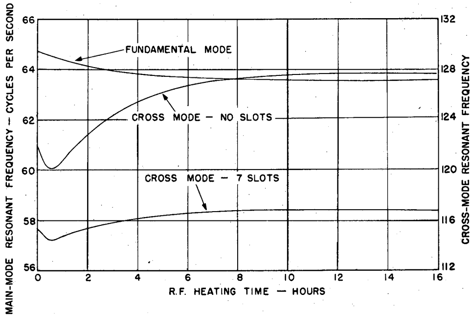
EFFECT OF TEMPERATURE ON REED RESONANT FREQUENCIES
