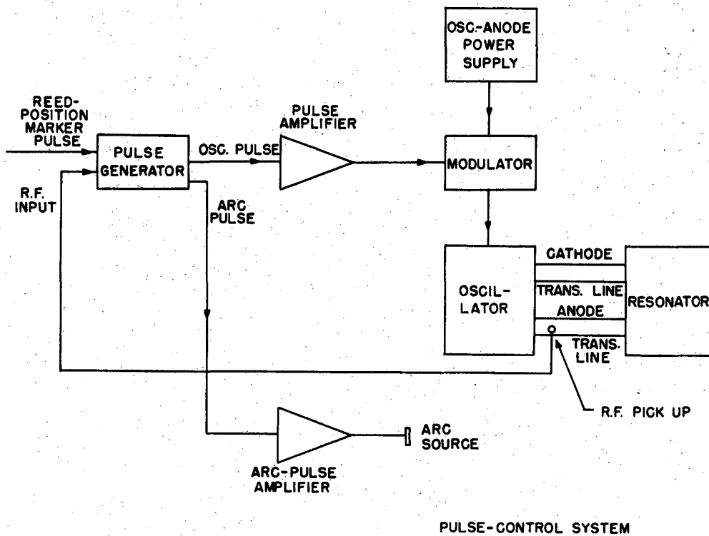
PULSE-CONTROL SYSTEM
